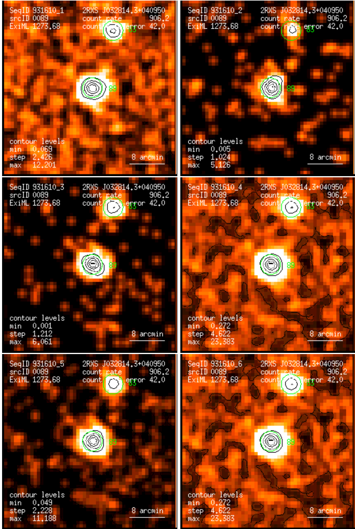
Figure 89: RASS 931610: detection 0089: band rate images, Gaussian filter: (1) PSPC channels 11 – 41, (2) 52 – 90, (3) 91 – 201, (4) 11 – 235, (5) 52 – 201, (6) 11 – 201. Broad band rates in counts/ks. Band rate contour levels in counts/ks/arcmin 2 .
