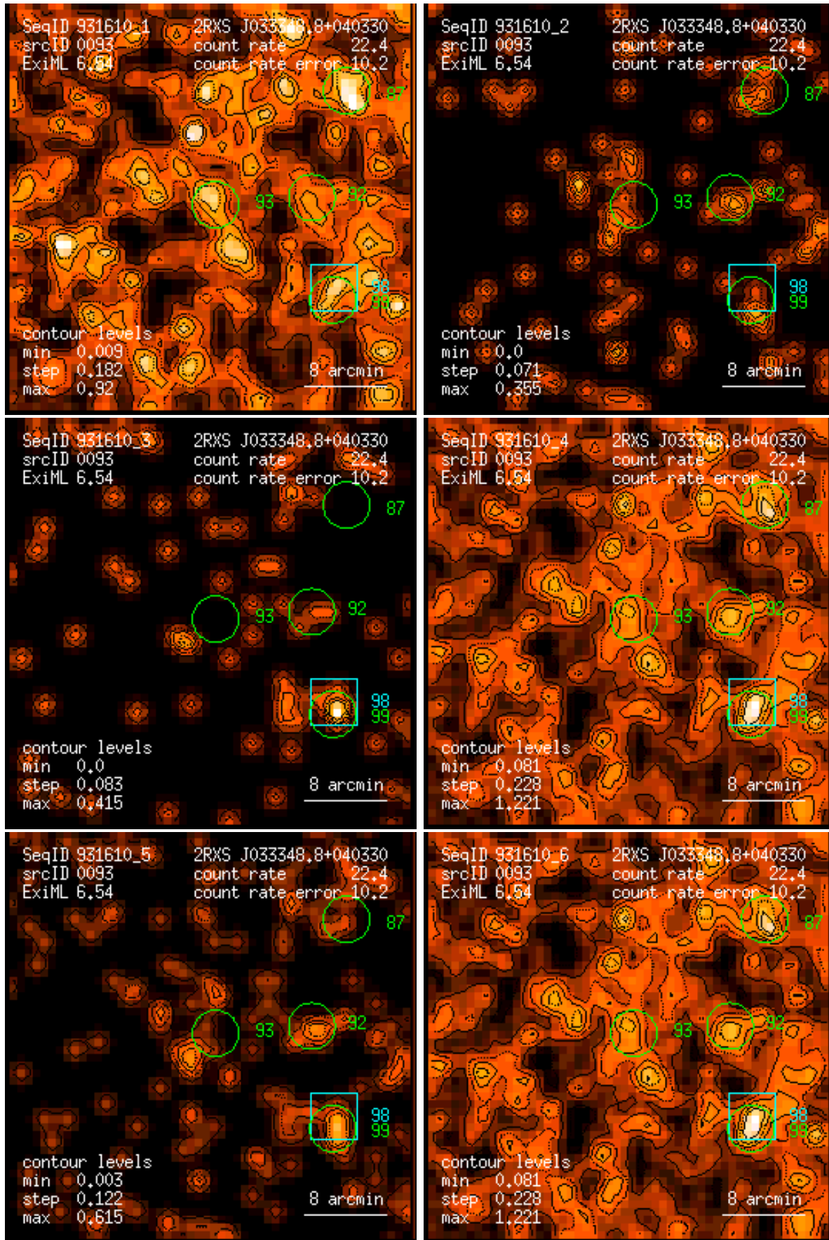
Figure 93: RASS 931610: detection 0093: band rate images, Gaussian filter: (1) PSPC channels 11 – 41, (2) 52 – 90, (3) 91 – 201, (4) 11 – 235, (5) 52 – 201, (6) 11 – 201. Broad band rates in counts/ks. Band rate contour levels in counts/ks/arcmin 2 .
