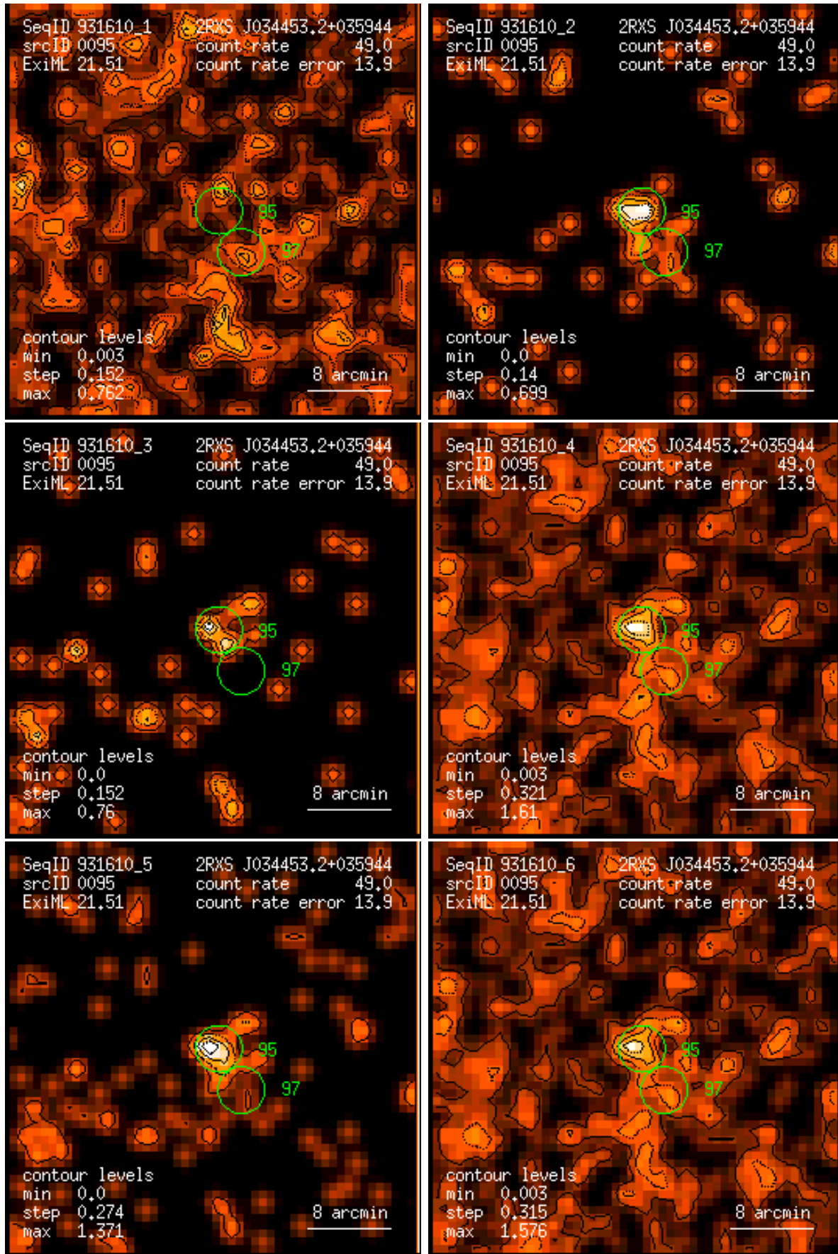
Figure 95: RASS 931610: detection 0095: band rate images, Gaussian filter: (1) PSPC channels 11 – 41, (2) 52 – 90, (3) 91 – 201, (4) 11 – 235, (5) 52 – 201, (6) 11 – 201. Broad band rates in counts/ks. Band rate contour levels in counts/ks/arcmin 2 .
