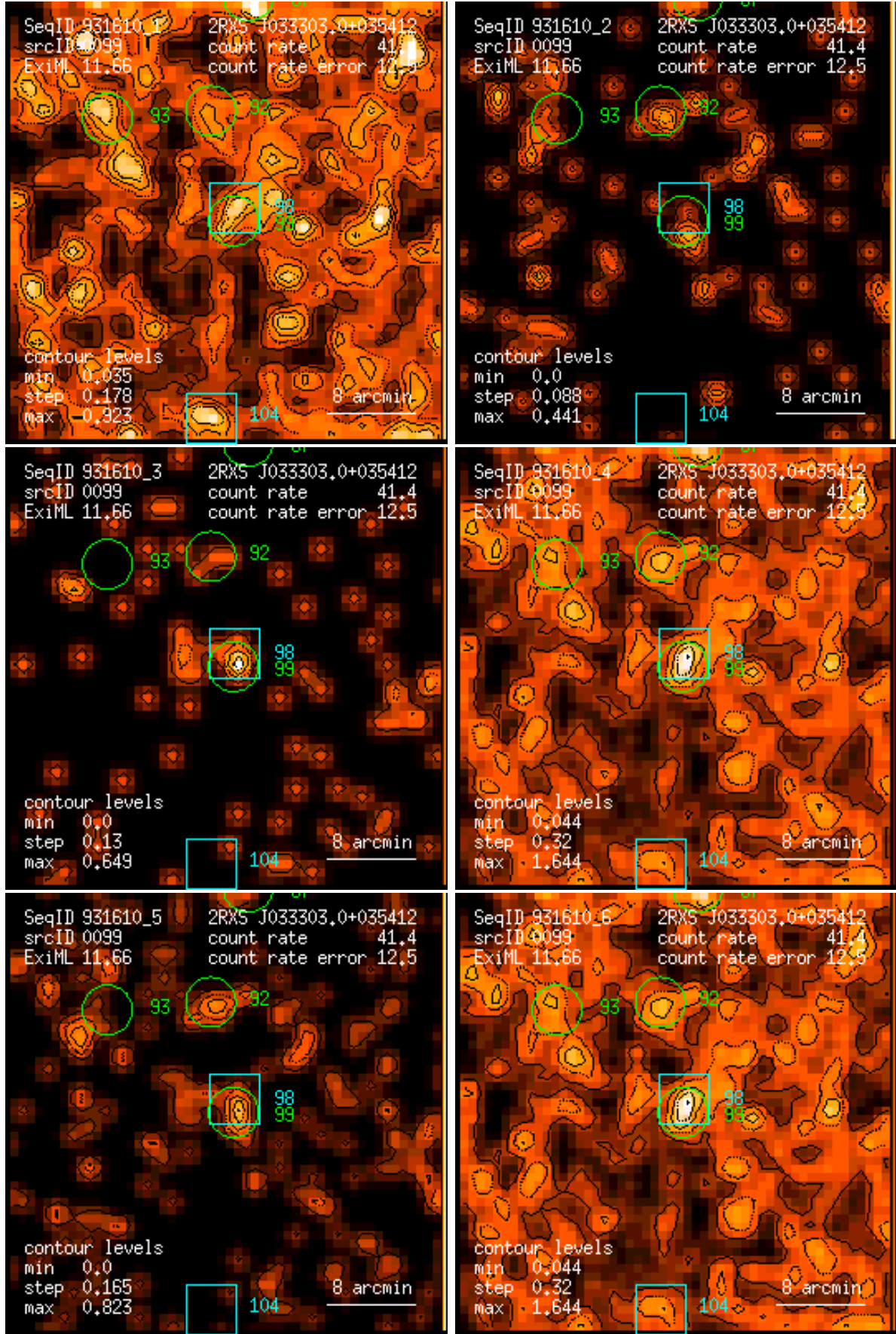
Figure 99: RASS 931610: detection 0099: band rate images, Gaussian filter: (1) PSPC channels 11 – 41, (2) 52 – 90, (3) 91 – 201, (4) 11 – 235, (5) 52 – 201, (6) 11 – 201. Broad band rates in counts/ks. Band rate contour levels in counts/ks/arcmin 2 .
