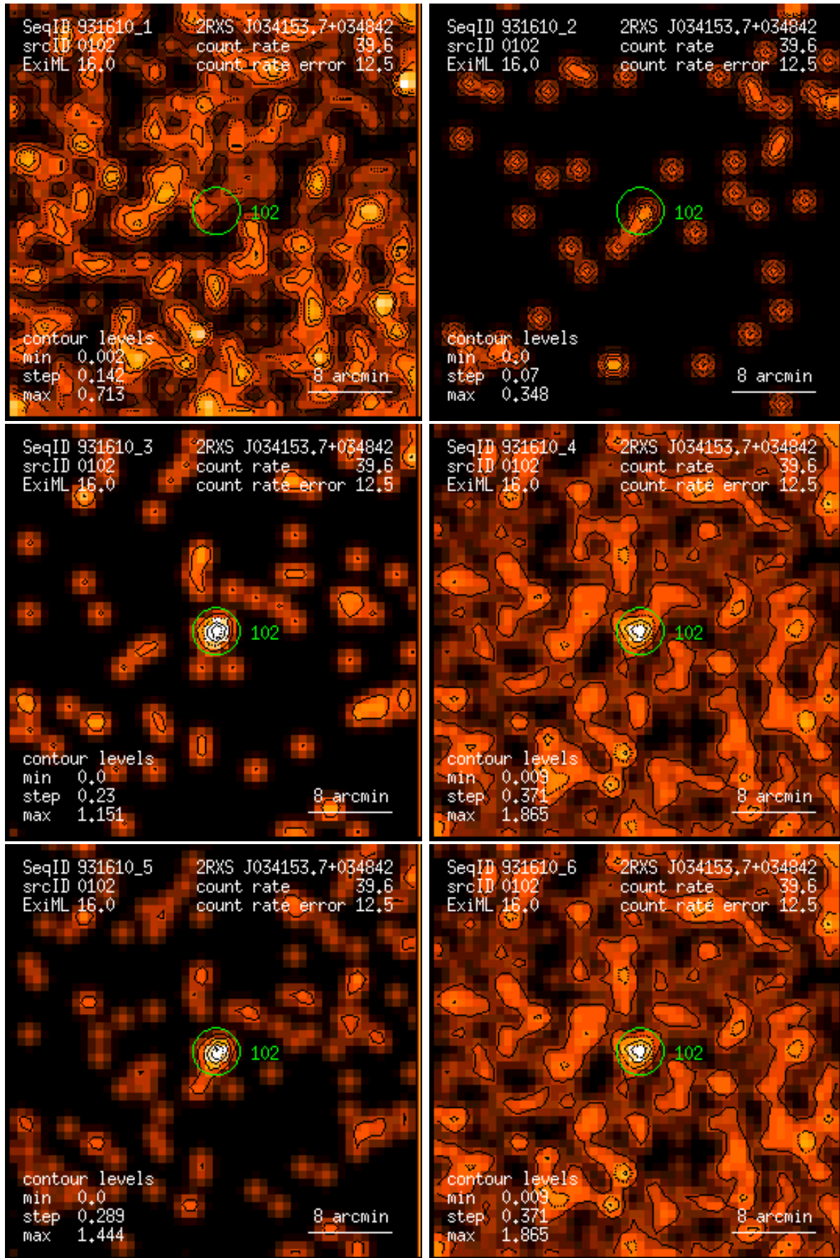
Figure 102: RASS 931610: detection 0102: band rate images, Gaussian filter: (1) PSPC channels 11 – 41, (2) 52 – 90, (3) 91 – 201, (4) 11 – 235, (5) 52 – 201, (6) 11 – 201. Broad band rates in counts/ks. Band rate contour levels in counts/ks/arcmin 2 .
