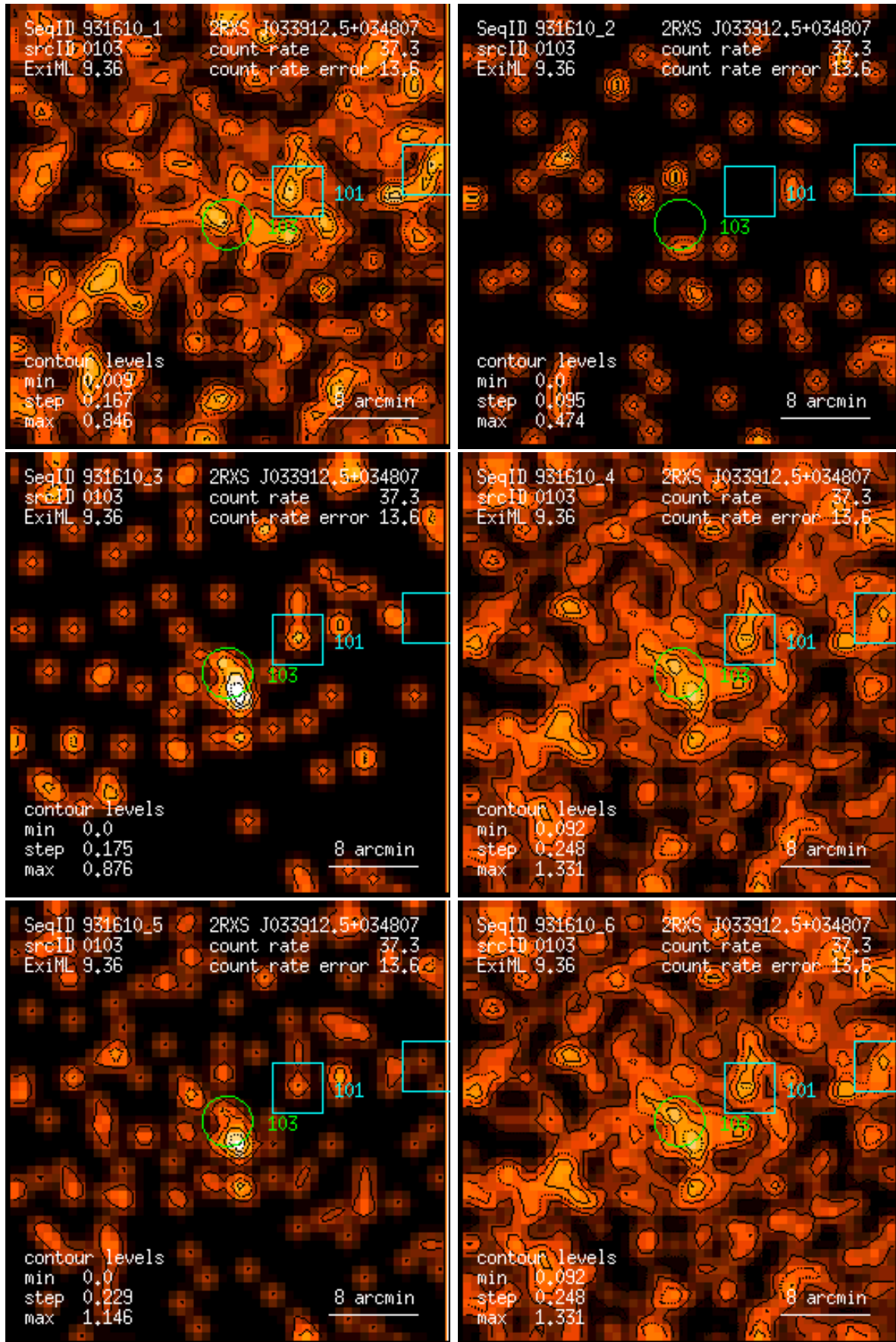
Figure 103: RASS 931610: detection 0103: band rate images, Gaussian filter: (1) PSPC channels 11 – 41, (2) 52 – 90, (3) 91 – 201, (4) 11 – 235, (5) 52 – 201, (6) 11 – 201. Broad band rates in counts/ks. Band rate contour levels in counts/ks/arcmin 2 .
