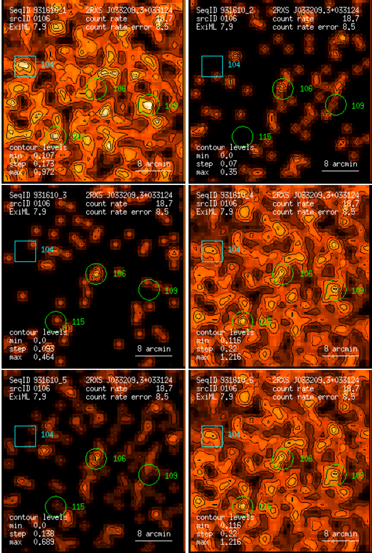
Figure 106: RASS 931610: detection 0106: band rate images, Gaussian filter: (1) PSPC channels 11 – 41, (2) 52 – 90, (3) 91 – 201, (4) 11 – 235, (5) 52 – 201, (6) 11 – 201. Broad band rates in counts/ks. Band rate contour levels in counts/ks/arcmin 2 .
