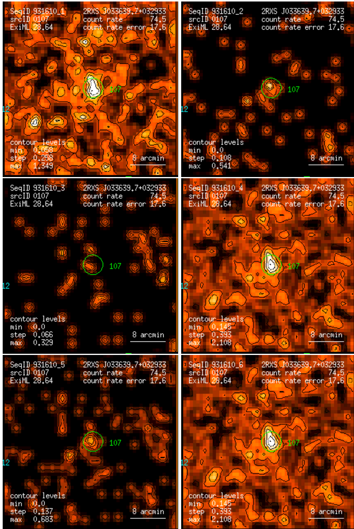
Figure 107: RASS 931610: detection 0107: band rate images, Gaussian filter: (1) PSPC channels 11 – 41, (2) 52 – 90, (3) 91 – 201, (4) 11 – 235, (5) 52 – 201, (6) 11 – 201. Broad band rates in counts/ks. Band rate contour levels in counts/ks/arcmin 2 .
