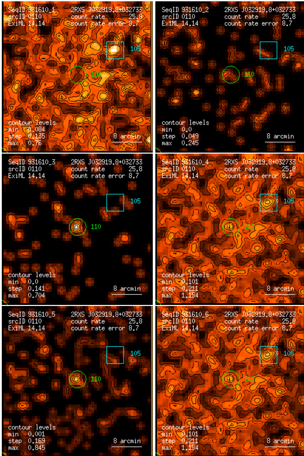
Figure 110: RASS 931610: detection 0110: band rate images, Gaussian filter: (1) PSPC channels 11 – 41, (2) 52 – 90, (3) 91 – 201, (4) 11 – 235, (5) 52 – 201, (6) 11 – 201. Broad band rates in counts/ks. Band rate contour levels in counts/ks/arcmin 2 .
