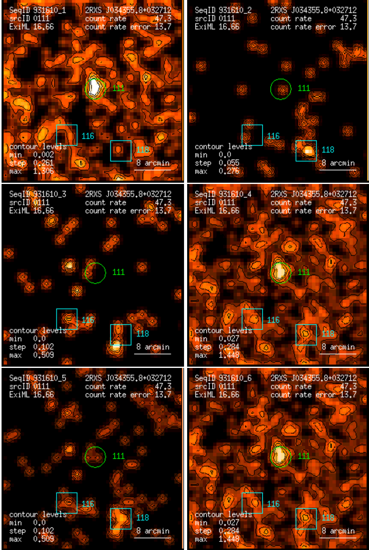
Figure 111: RASS 931610: detection 0111: band rate images, Gaussian filter: (1) PSPC channels 11 – 41, (2) 52 – 90, (3) 91 – 201, (4) 11 – 235, (5) 52 – 201, (6) 11 – 201. Broad band rates in counts/ks. Band rate contour levels in counts/ks/arcmin 2 .
