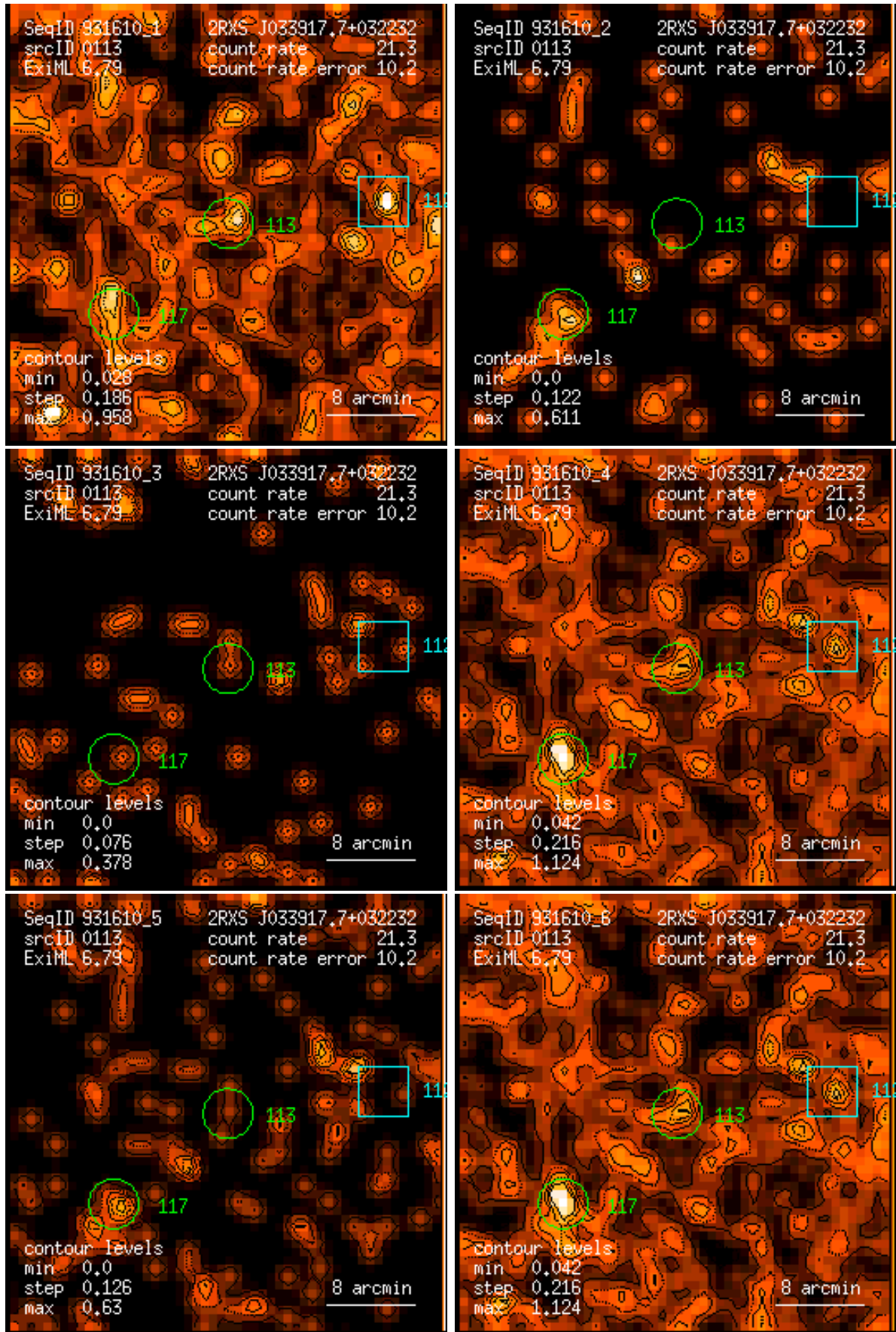
Figure 113: RASS 931610: detection 0113: band rate images, Gaussian filter: (1) PSPC channels 11 – 41, (2) 52 – 90, (3) 91 – 201, (4) 11 – 235, (5) 52 – 201, (6) 11 – 201. Broad band rates in counts/ks. Band rate contour levels in counts/ks/arcmin 2 .
