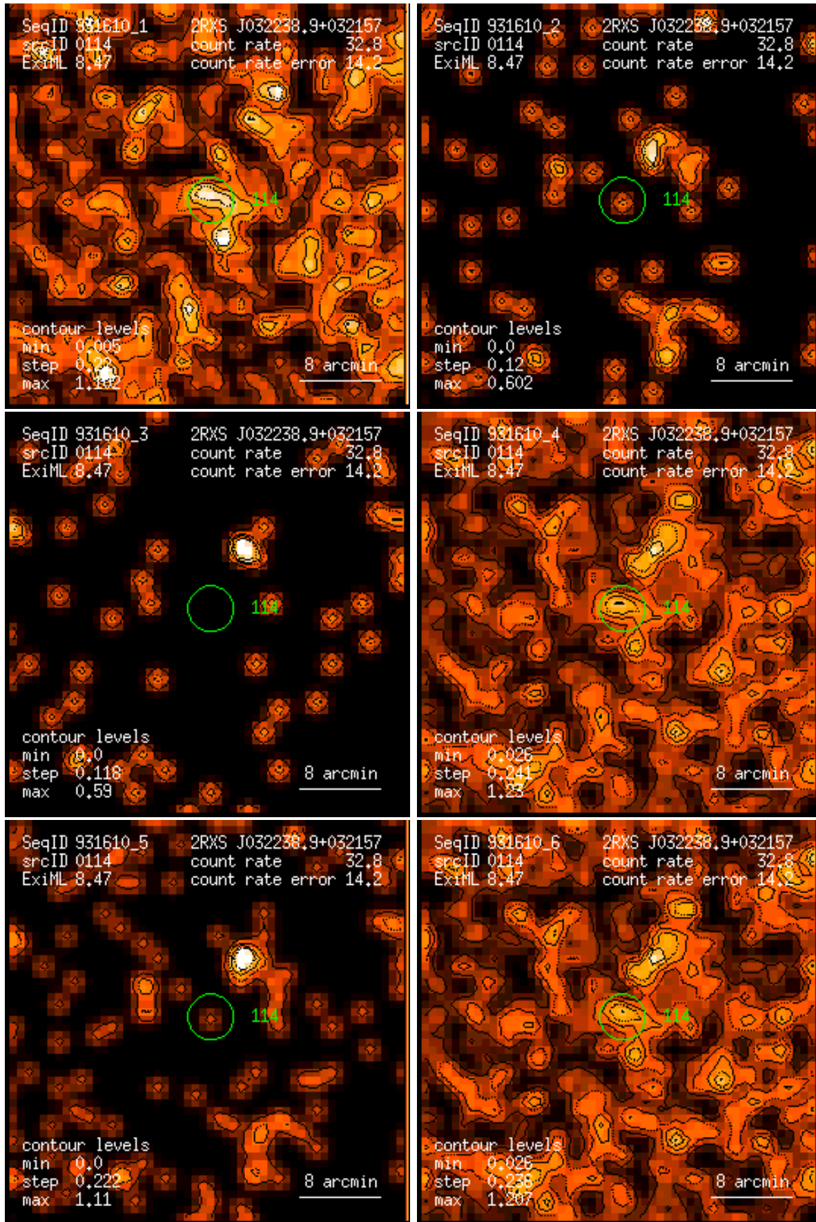
Figure 114: RASS 931610: detection 0114: band rate images, Gaussian filter: (1) PSPC channels 11 – 41, (2) 52 – 90, (3) 91 – 201, (4) 11 – 235, (5) 52 – 201, (6) 11 – 201. Broad band rates in counts/ks. Band rate contour levels in counts/ks/arcmin 2 .
