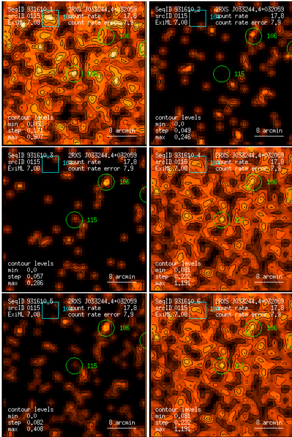
Figure 115: RASS 931610: detection 0115: band rate images, Gaussian filter: (1) PSPC channels 11 – 41, (2) 52 – 90, (3) 91 – 201, (4) 11 – 235, (5) 52 – 201, (6) 11 – 201. Broad band rates in counts/ks. Band rate contour levels in counts/ks/arcmin 2 .
