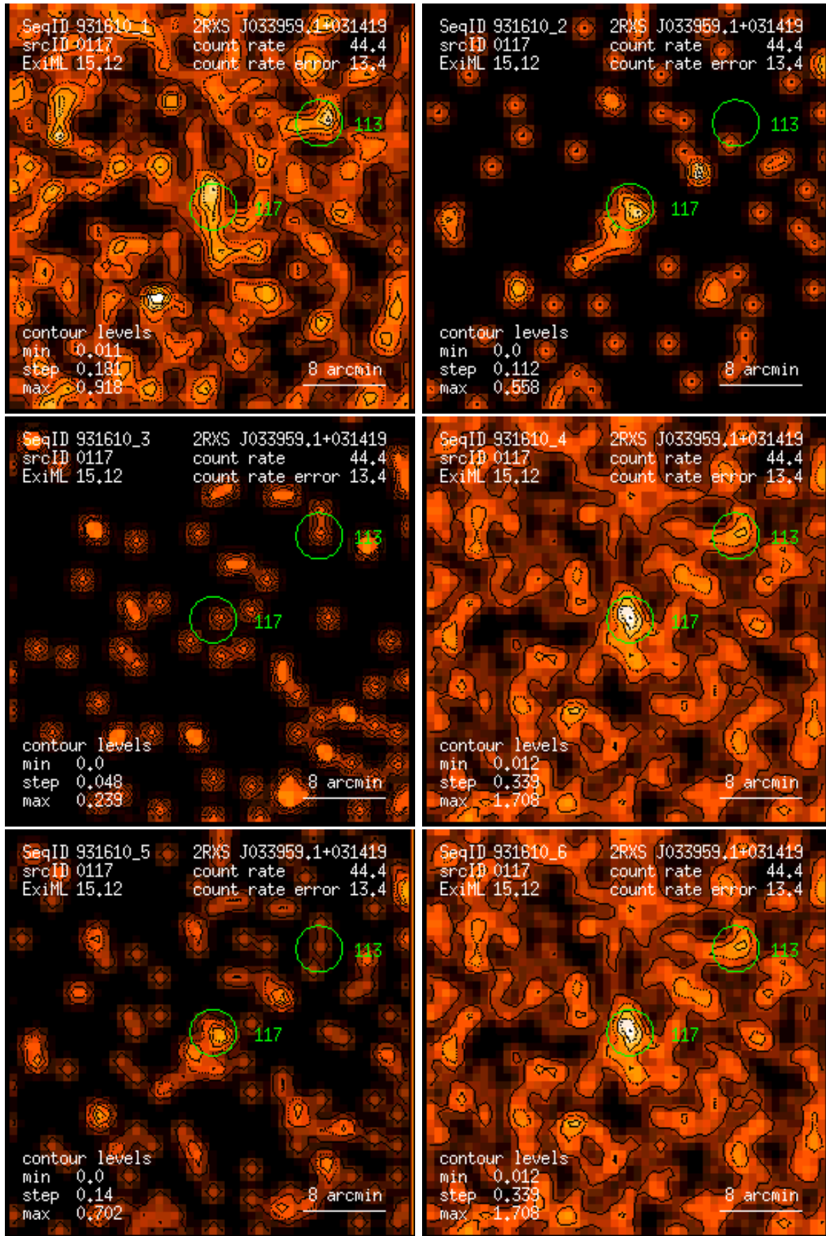
Figure 117: RASS 931610: detection 0117: band rate images, Gaussian filter: (1) PSPC channels 11 – 41, (2) 52 – 90, (3) 91 – 201, (4) 11 – 235, (5) 52 – 201, (6) 11 – 201. Broad band rates in counts/ks. Band rate contour levels in counts/ks/arcmin 2 .
