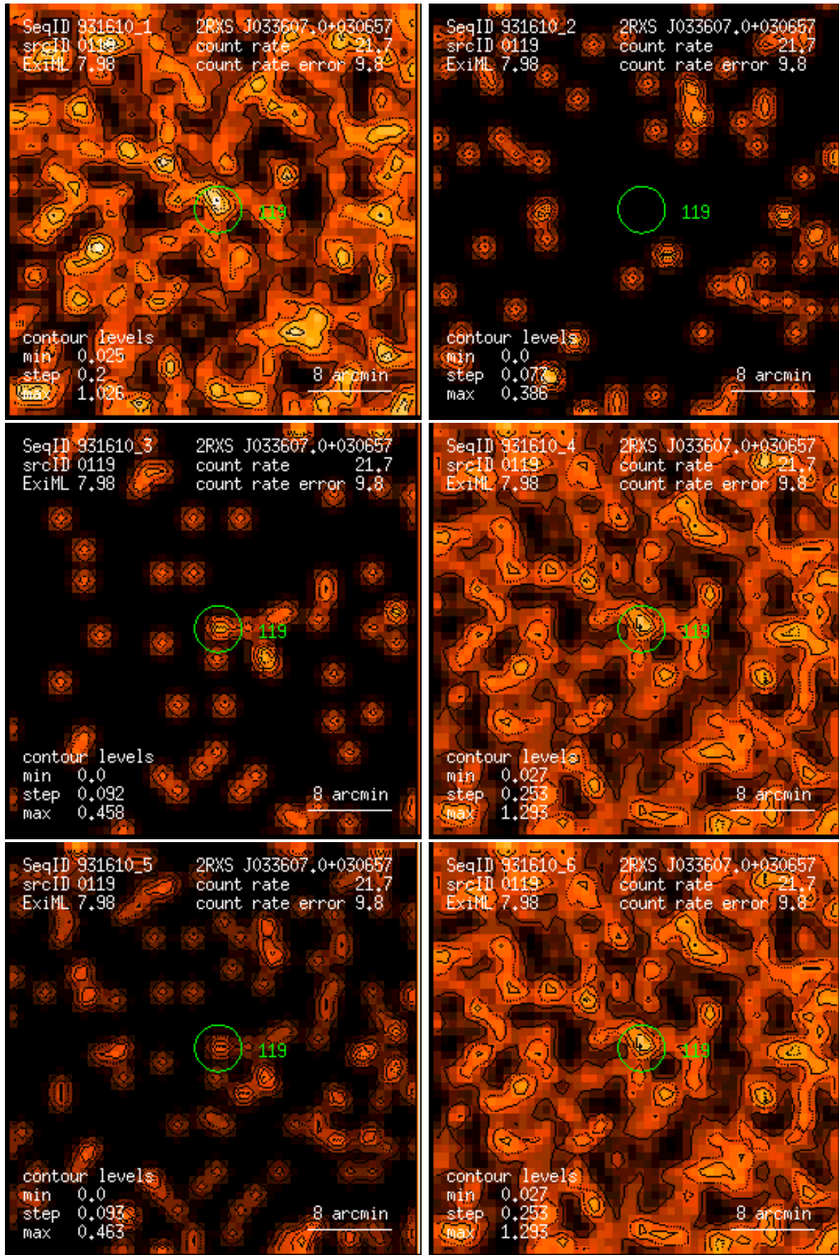
Figure 119: RASS 931610: detection 0119: band rate images, Gaussian filter: (1) PSPC channels 11 – 41, (2) 52 – 90, (3) 91 – 201, (4) 11 – 235, (5) 52 – 201, (6) 11 – 201. Broad band rates in counts/ks. Band rate contour levels in counts/ks/arcmin 2 .
