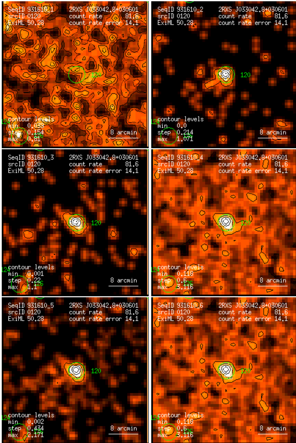
Figure 120: RASS 931610: detection 0120: band rate images, Gaussian filter: (1) PSPC channels 11 – 41, (2) 52 – 90, (3) 91 – 201, (4) 11 – 235, (5) 52 – 201, (6) 11 – 201. Broad band rates in counts/ks. Band rate contour levels in counts/ks/arcmin 2 .
