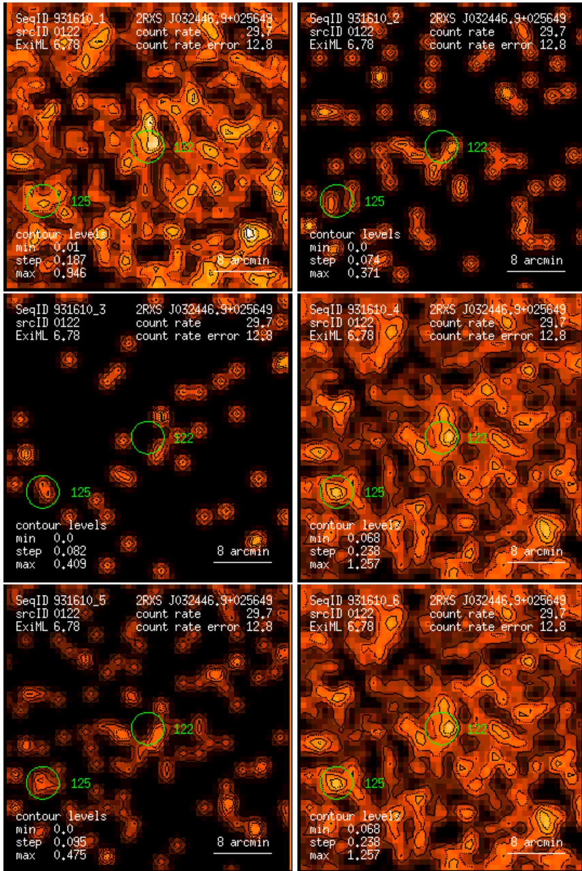
Figure 122: RASS 931610: detection 0122: band rate images, Gaussian filter: (1) PSPC channels 11 – 41, (2) 52 – 90, (3) 91 – 201, (4) 11 – 235, (5) 52 – 201, (6) 11 – 201. Broad band rates in counts/ks. Band rate contour levels in counts/ks/arcmin 2 .
