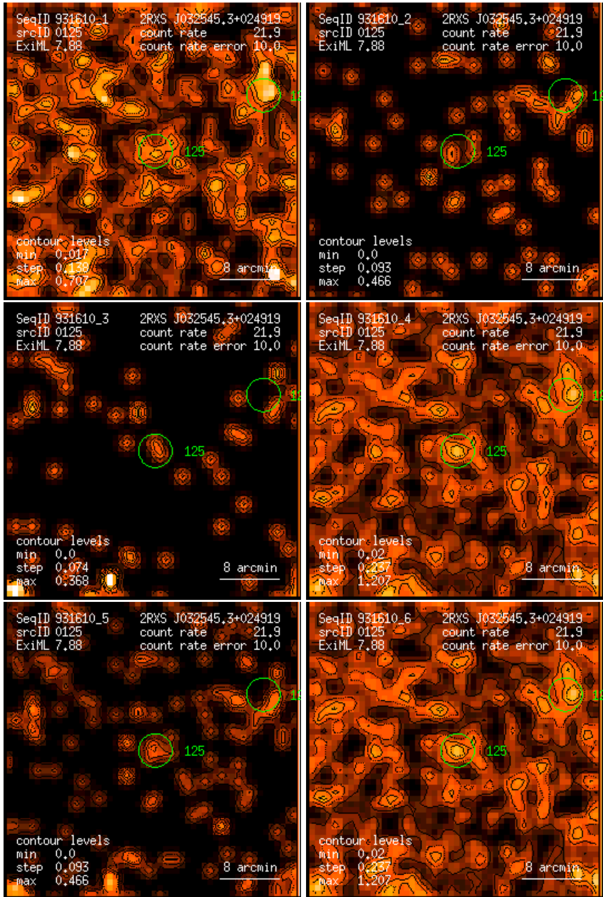
Figure 125: RASS 931610: detection 0125: band rate images, Gaussian filter: (1) PSPC channels 11 – 41, (2) 52 – 90, (3) 91 – 201, (4) 11 – 235, (5) 52 – 201, (6) 11 – 201. Broad band rates in counts/ks. Band rate contour levels in counts/ks/arcmin 2 .
