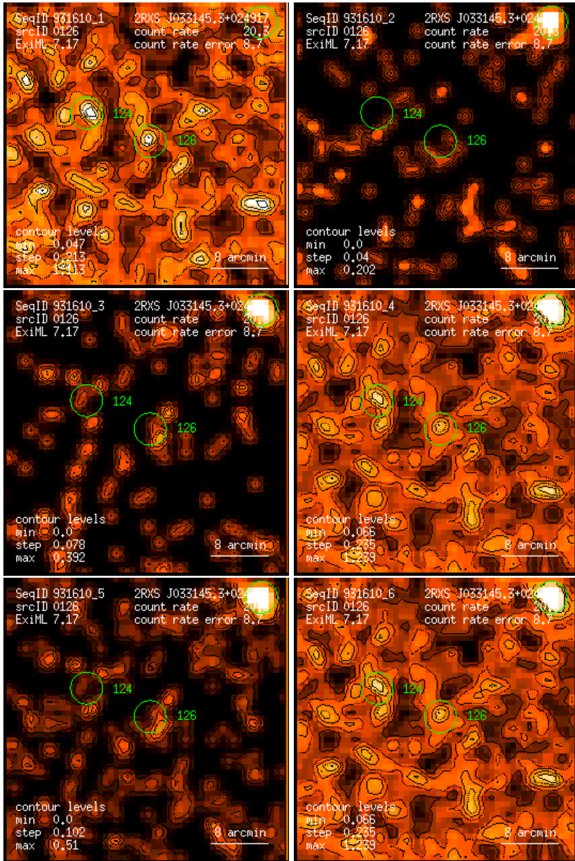
Figure 126: RASS 931610: detection 0126: band rate images, Gaussian filter: (1) PSPC channels 11 – 41, (2) 52 – 90, (3) 91 – 201, (4) 11 – 235, (5) 52 – 201, (6) 11 – 201. Broad band rates in counts/ks. Band rate contour levels in counts/ks/arcmin 2 .
