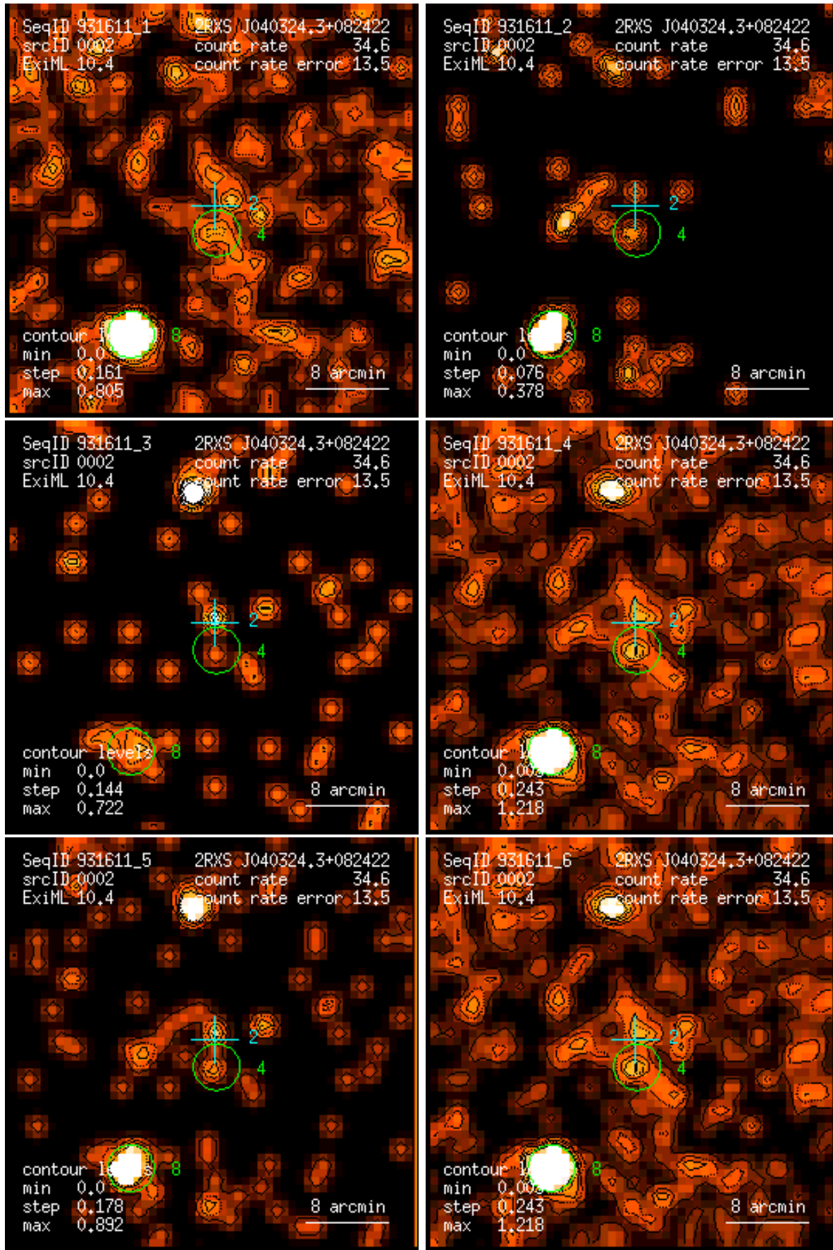
Figure 2: RASS 931611: detection 0002: band rate images, Gaussian filter: (1) PSPC channels 11 – 41, (2) 52 – 90, (3) 91 – 201, (4) 11 – 235, (5) 52 – 201, (6) 11 – 201. Broad band rates in counts/ks. Band rate contour levels in counts/ks/arcmin 2 .
