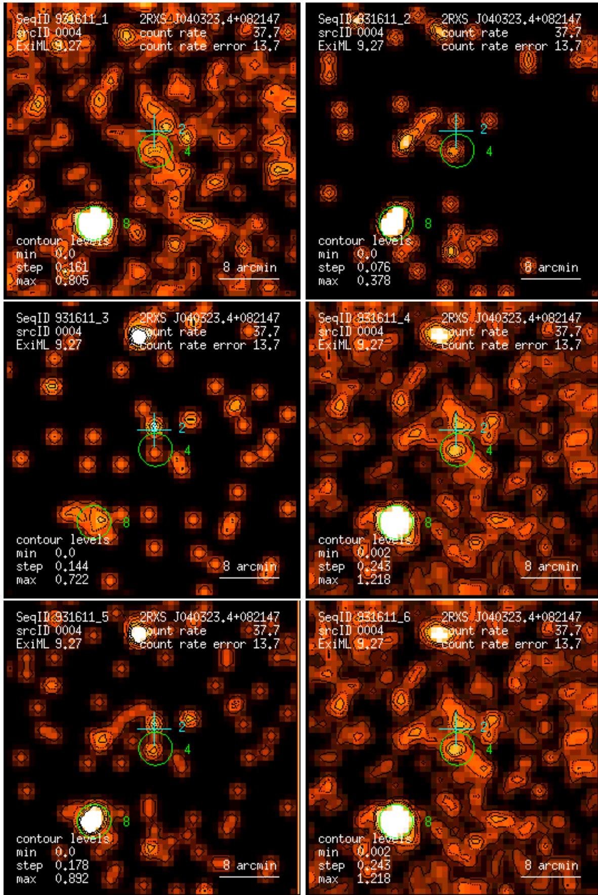
Figure 4: RASS 931611: detection 0004: band rate images, Gaussian filter: (1) PSPC channels 11 – 41, (2) 52 – 90, (3) 91 – 201, (4) 11 – 235, (5) 52 – 201, (6) 11 – 201. Broad band rates in counts/ks. Band rate contour levels in counts/ks/arcmin 2 .
