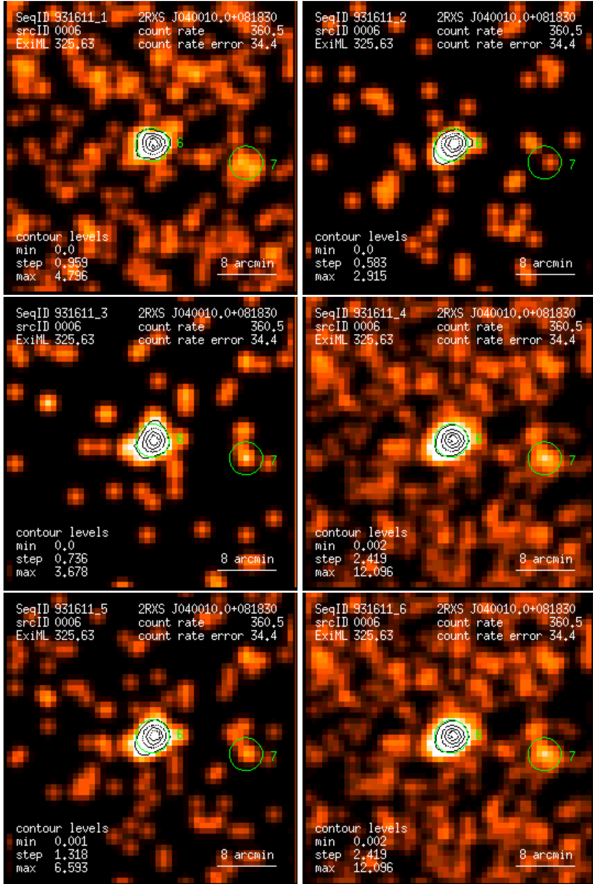
Figure 6: RASS 931611: detection 0006: band rate images, Gaussian filter: (1) PSPC channels 11 – 41, (2) 52 – 90, (3) 91 – 201, (4) 11 – 235, (5) 52 – 201, (6) 11 – 201. Broad band rates in counts/ks. Band rate contour levels in counts/ks/arcmin 2 .
