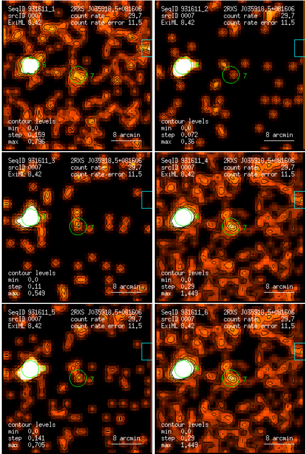
Figure 7: RASS 931611: detection 0007: band rate images, Gaussian filter: (1) PSPC channels 11 – 41, (2) 52 – 90, (3) 91 – 201, (4) 11 – 235, (5) 52 – 201, (6) 11 – 201. Broad band rates in counts/ks. Band rate contour levels in counts/ks/arcmin 2 .
