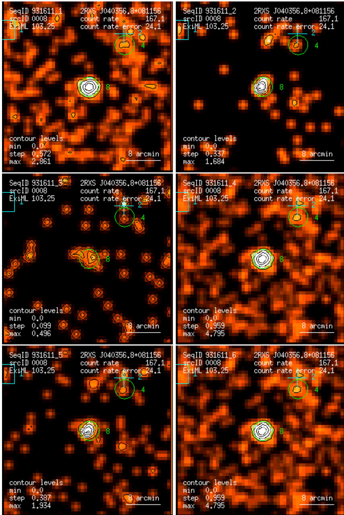
Figure 8: RASS 931611: detection 0008: band rate images, Gaussian filter: (1) PSPC channels 11 – 41, (2) 52 – 90, (3) 91 – 201, (4) 11 – 235, (5) 52 – 201, (6) 11 – 201. Broad band rates in counts/ks. Band rate contour levels in counts/ks/arcmin 2 .
