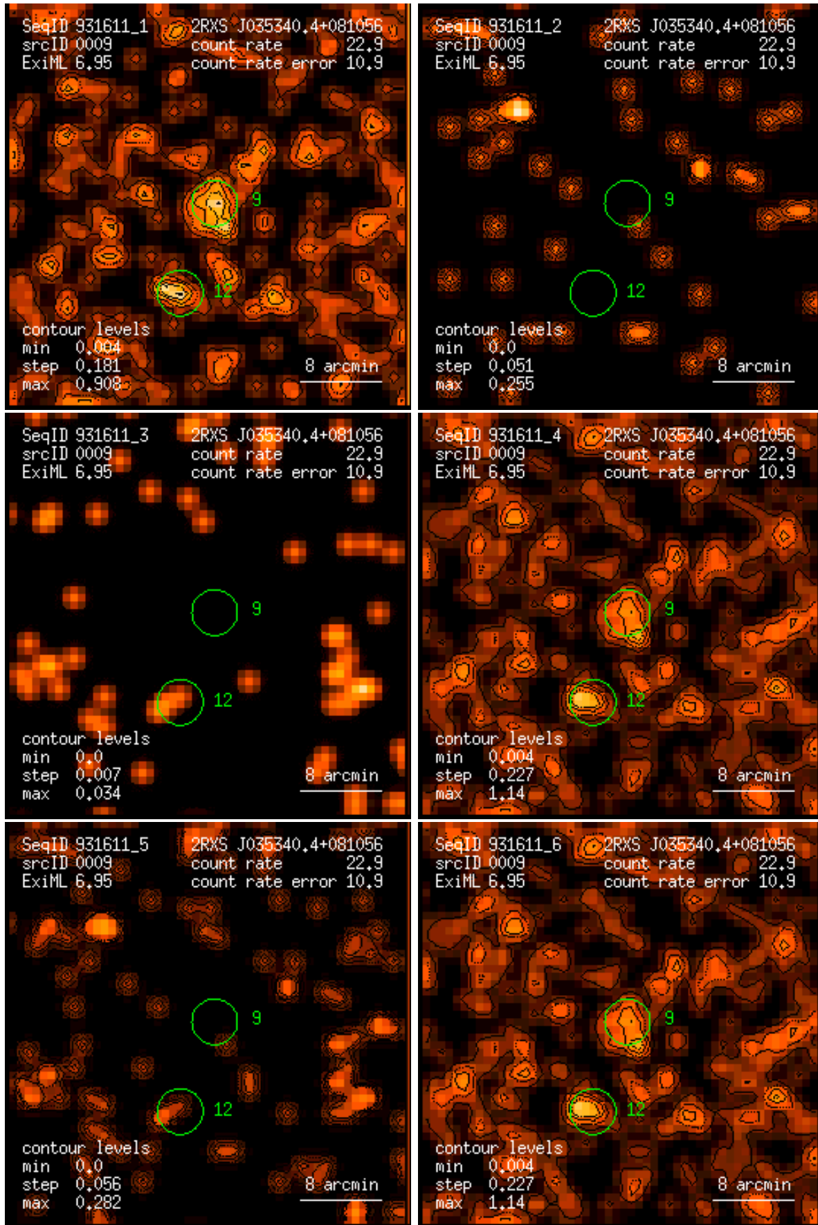
Figure 9: RASS 931611: detection 0009: band rate images, Gaussian filter: (1) PSPC channels 11 – 41, (2) 52 – 90, (3) 91 – 201, (4) 11 – 235, (5) 52 – 201, (6) 11 – 201. Broad band rates in counts/ks. Band rate contour levels in counts/ks/arcmin 2 .
