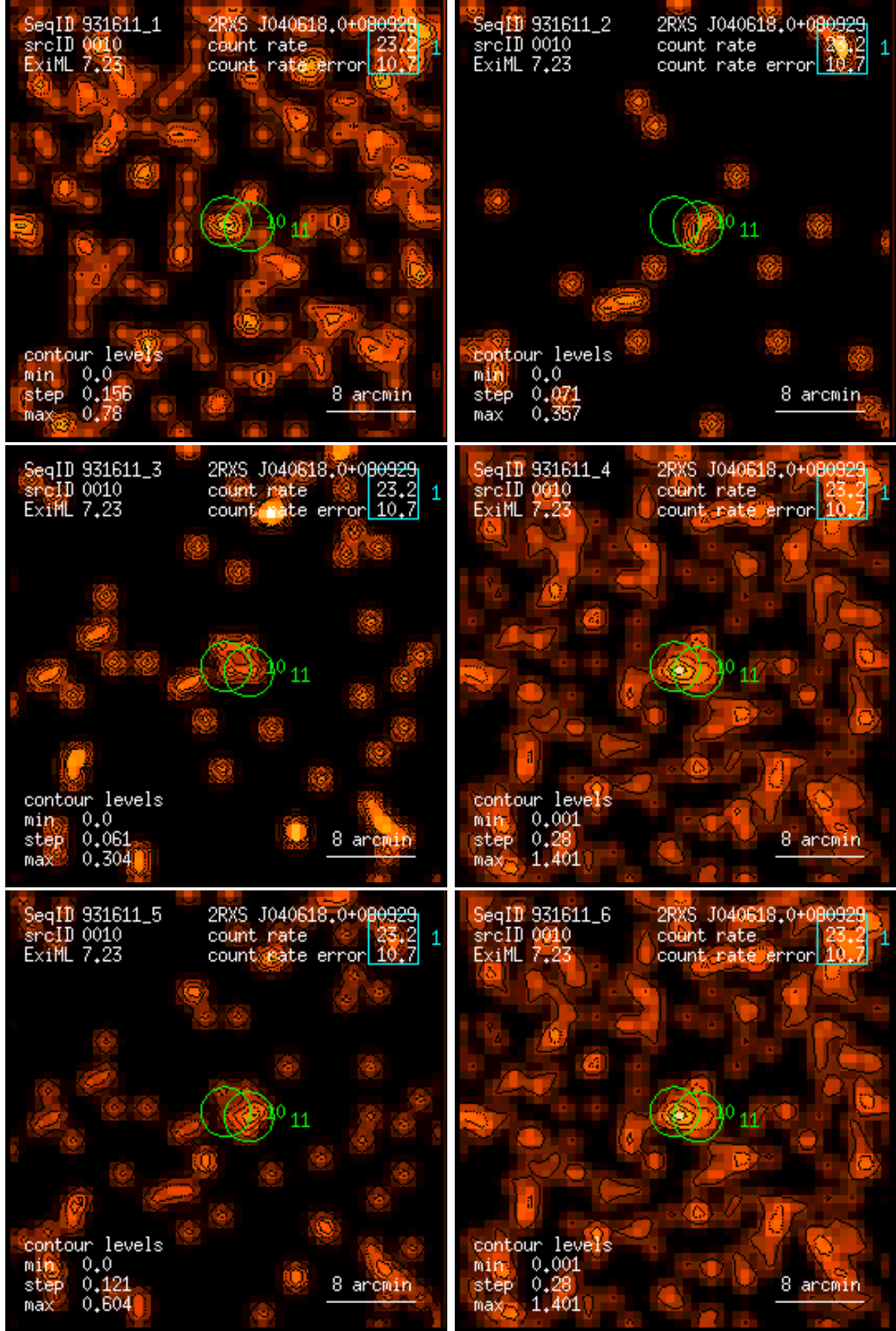
Figure 10: RASS 931611: detection 0010: band rate images, Gaussian filter: (1) PSPC channels 11 – 41, (2) 52 – 90, (3) 91 – 201, (4) 11 – 235, (5) 52 – 201, (6) 11 – 201. Broad band rates in counts/ks. Band rate contour levels in counts/ks/arcmin 2 .
