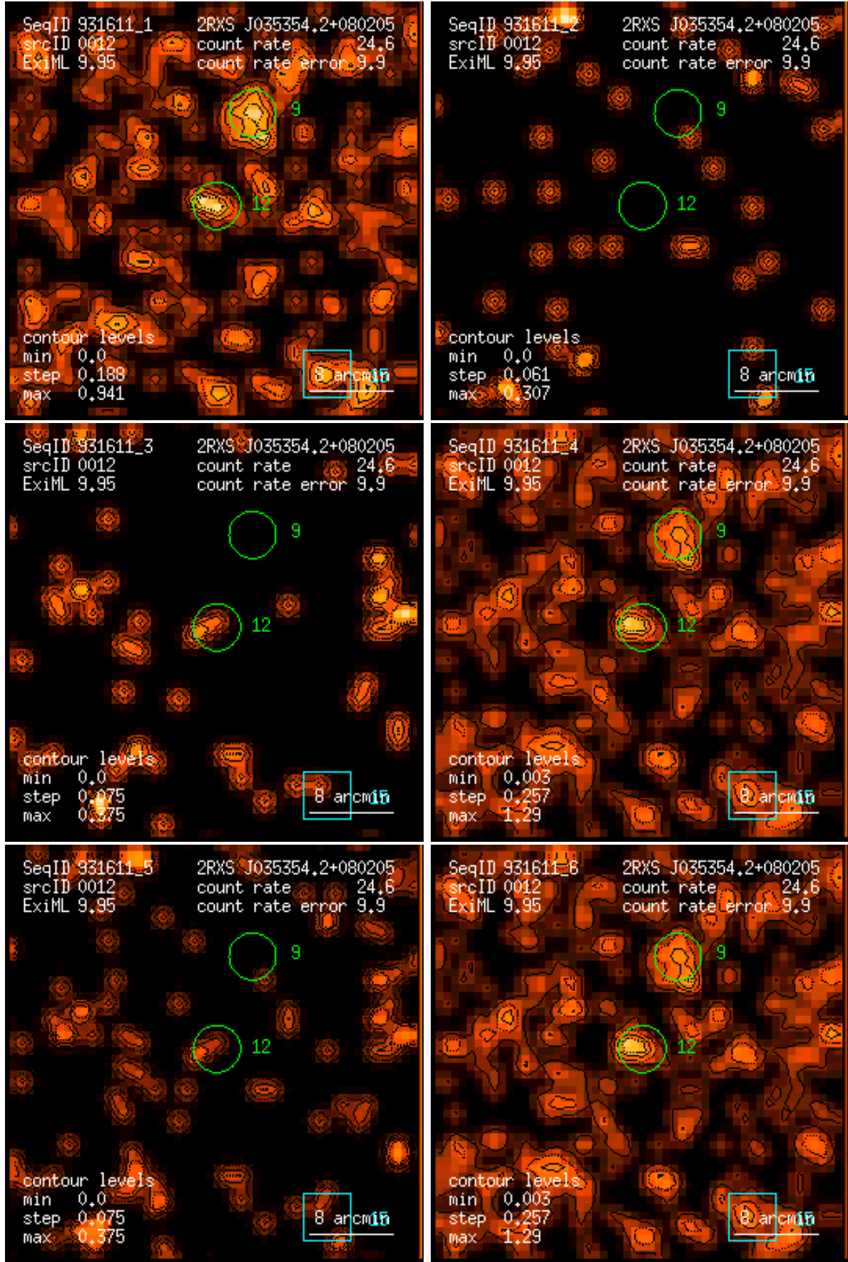
Figure 12: RASS 931611: detection 0012: band rate images, Gaussian filter: (1) PSPC channels 11 – 41, (2) 52 – 90, (3) 91 – 201, (4) 11 – 235, (5) 52 – 201, (6) 11 – 201. Broad band rates in counts/ks. Band rate contour levels in counts/ks/arcmin 2 .
