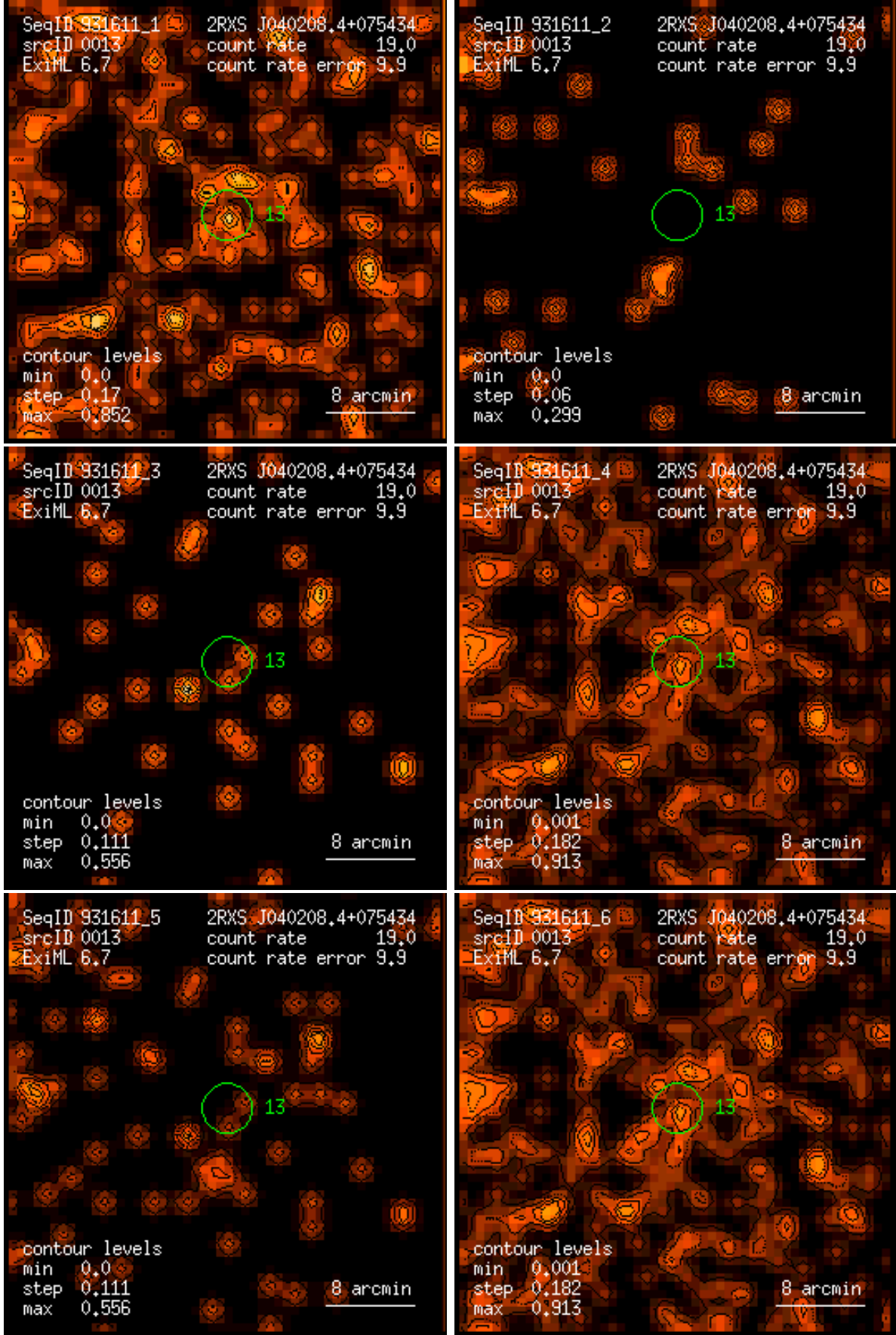
Figure 13: RASS 931611: detection 0013: band rate images, Gaussian filter: (1) PSPC channels 11 – 41, (2) 52 – 90, (3) 91 – 201, (4) 11 – 235, (5) 52 – 201, (6) 11 – 201. Broad band rates in counts/ks. Band rate contour levels in counts/ks/arcmin 2 .
