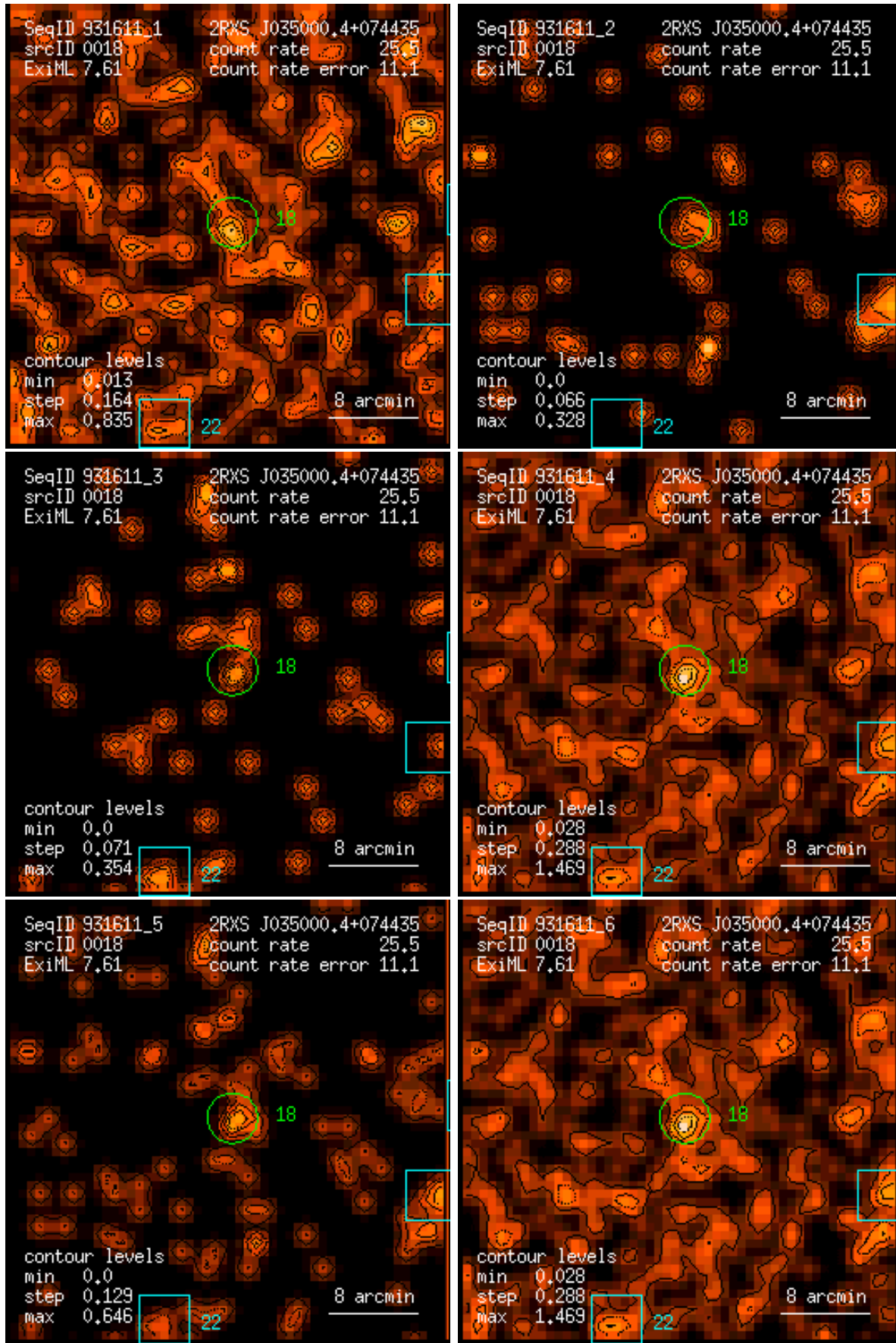
Figure 18: RASS 931611: detection 0018: band rate images, Gaussian filter: (1) PSPC channels 11 – 41, (2) 52 – 90, (3) 91 – 201, (4) 11 – 235, (5) 52 – 201, (6) 11 – 201. Broad band rates in counts/ks. Band rate contour levels in counts/ks/arcmin 2 .
