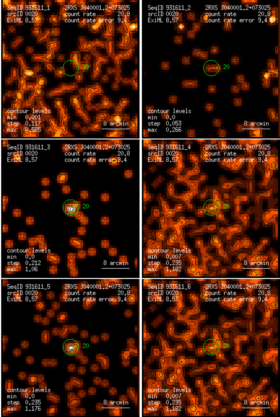
Figure 20: RASS 931611: detection 0020: band rate images, Gaussian filter: (1) PSPC channels 11 – 41, (2) 52 – 90, (3) 91 – 201, (4) 11 – 235, (5) 52 – 201, (6) 11 – 201. Broad band rates in counts/ks. Band rate contour levels in counts/ks/arcmin 2 .
