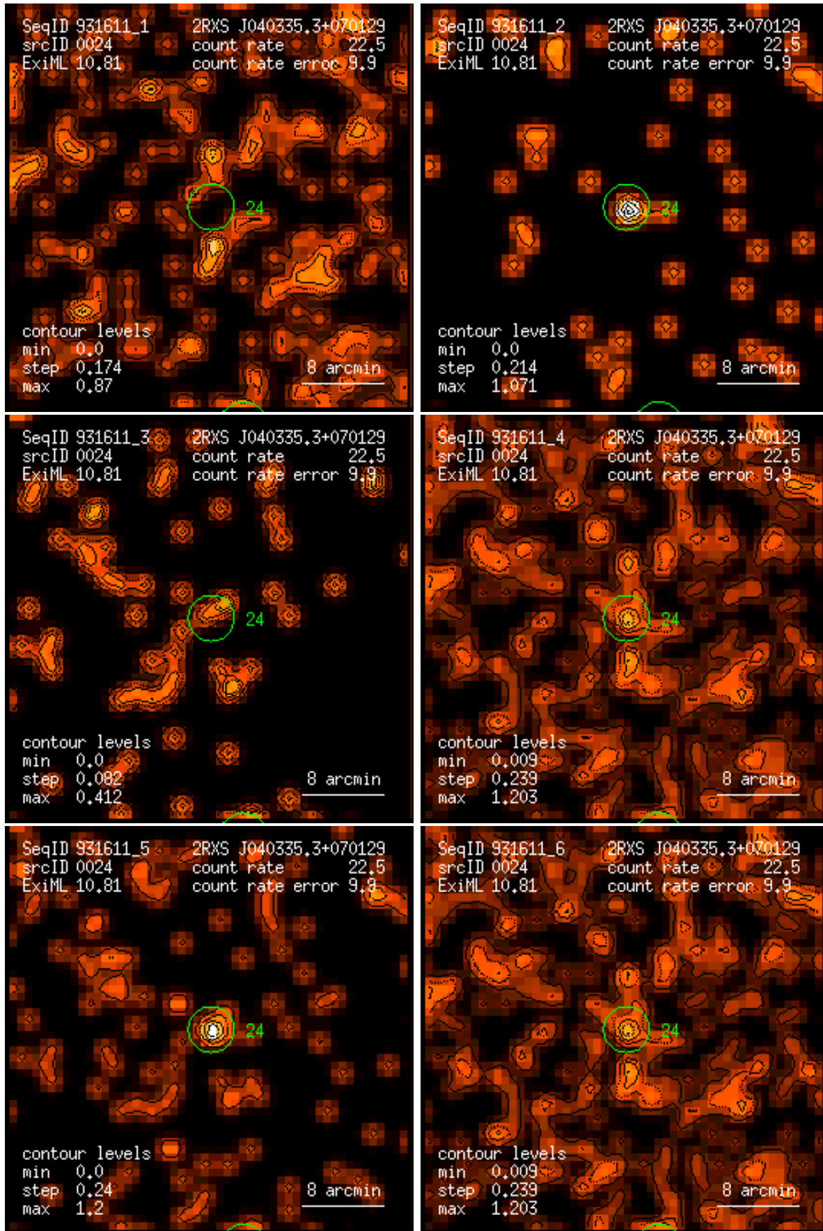
Figure 24: RASS 931611: detection 0024: band rate images, Gaussian filter: (1) PSPC channels 11 – 41, (2) 52 – 90, (3) 91 – 201, (4) 11 – 235, (5) 52 – 201, (6) 11 – 201. Broad band rates in counts/ks. Band rate contour levels in counts/ks/arcmin 2 .
