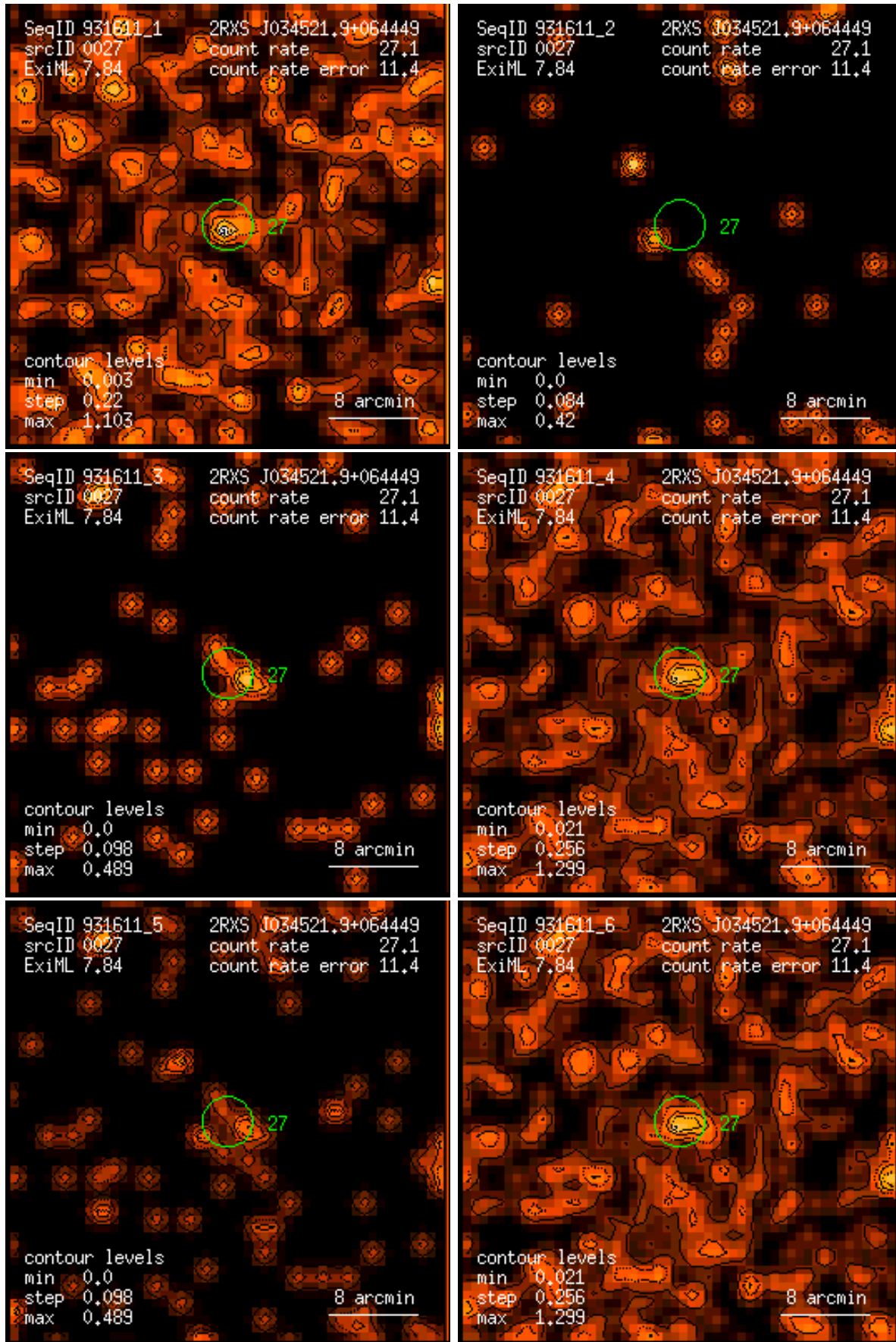
Figure 27: RASS 931611: detection 0027: band rate images, Gaussian filter: (1) PSPC channels 11 – 41, (2) 52 – 90, (3) 91 – 201, (4) 11 – 235, (5) 52 – 201, (6) 11 – 201. Broad band rates in counts/ks. Band rate contour levels in counts/ks/arcmin 2 .
