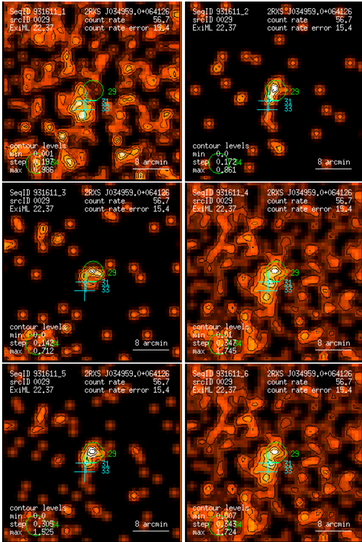
Figure 29: RASS 931611: detection 0029: band rate images, Gaussian filter: (1) PSPC channels 11 – 41, (2) 52 – 90, (3) 91 – 201, (4) 11 – 235, (5) 52 – 201, (6) 11 – 201. Broad band rates in counts/ks. Band rate contour levels in counts/ks/arcmin 2 .
