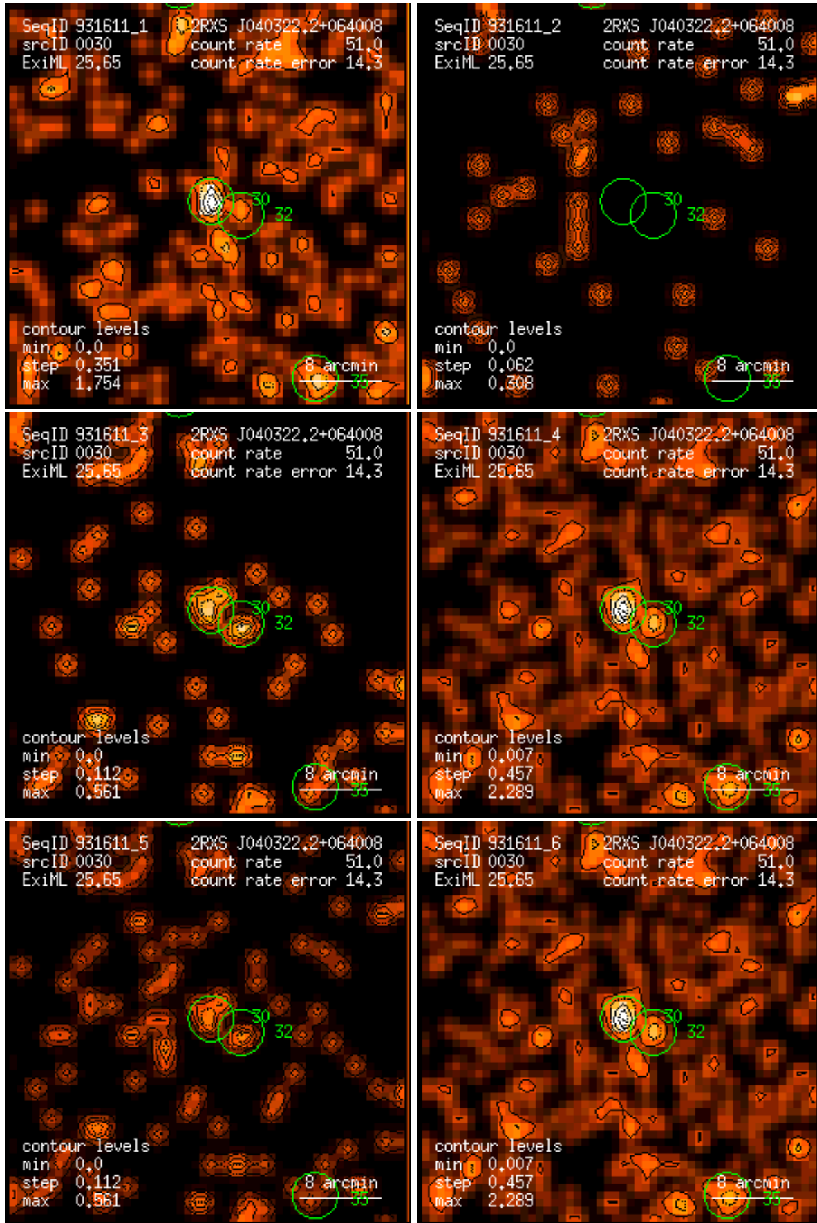
Figure 30: RASS 931611: detection 0030: band rate images, Gaussian filter: (1) PSPC channels 11 – 41, (2) 52 – 90, (3) 91 – 201, (4) 11 – 235, (5) 52 – 201, (6) 11 – 201. Broad band rates in counts/ks. Band rate contour levels in counts/ks/arcmin 2 .
