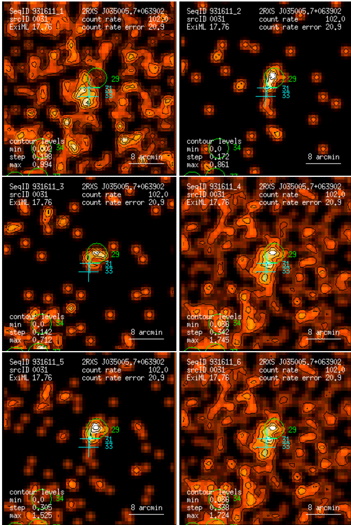
Figure 31: RASS 931611: detection 0031: band rate images, Gaussian filter: (1) PSPC channels 11 – 41, (2) 52 – 90, (3) 91 – 201, (4) 11 – 235, (5) 52 – 201, (6) 11 – 201. Broad band rates in counts/ks. Band rate contour levels in counts/ks/arcmin 2 .
