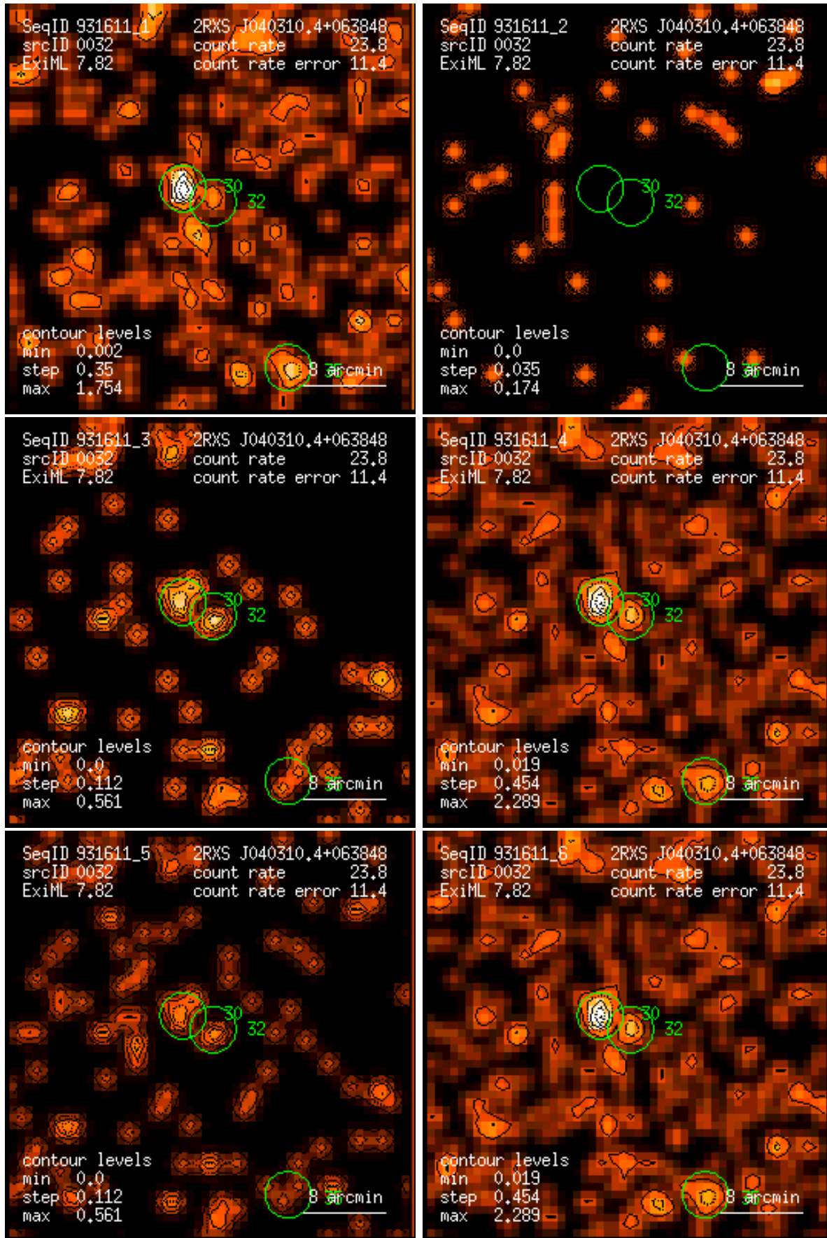
Figure 32: RASS 931611: detection 0032: band rate images, Gaussian filter: (1) PSPC channels 11 – 41, (2) 52 – 90, (3) 91 – 201, (4) 11 – 235, (5) 52 – 201, (6) 11 – 201. Broad band rates in counts/ks. Band rate contour levels in counts/ks/arcmin 2 .
