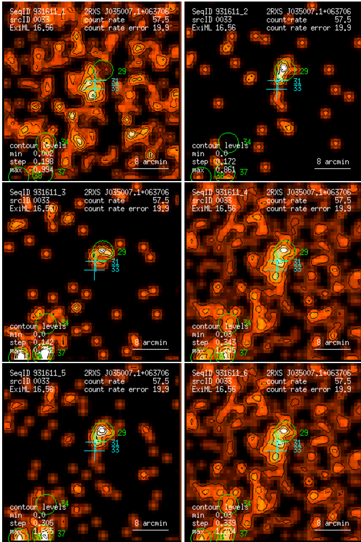
Figure 33: RASS 931611: detection 0033: band rate images, Gaussian filter: (1) PSPC channels 11 – 41, (2) 52 – 90, (3) 91 – 201, (4) 11 – 235, (5) 52 – 201, (6) 11 – 201. Broad band rates in counts/ks. Band rate contour levels in counts/ks/arcmin 2 .
