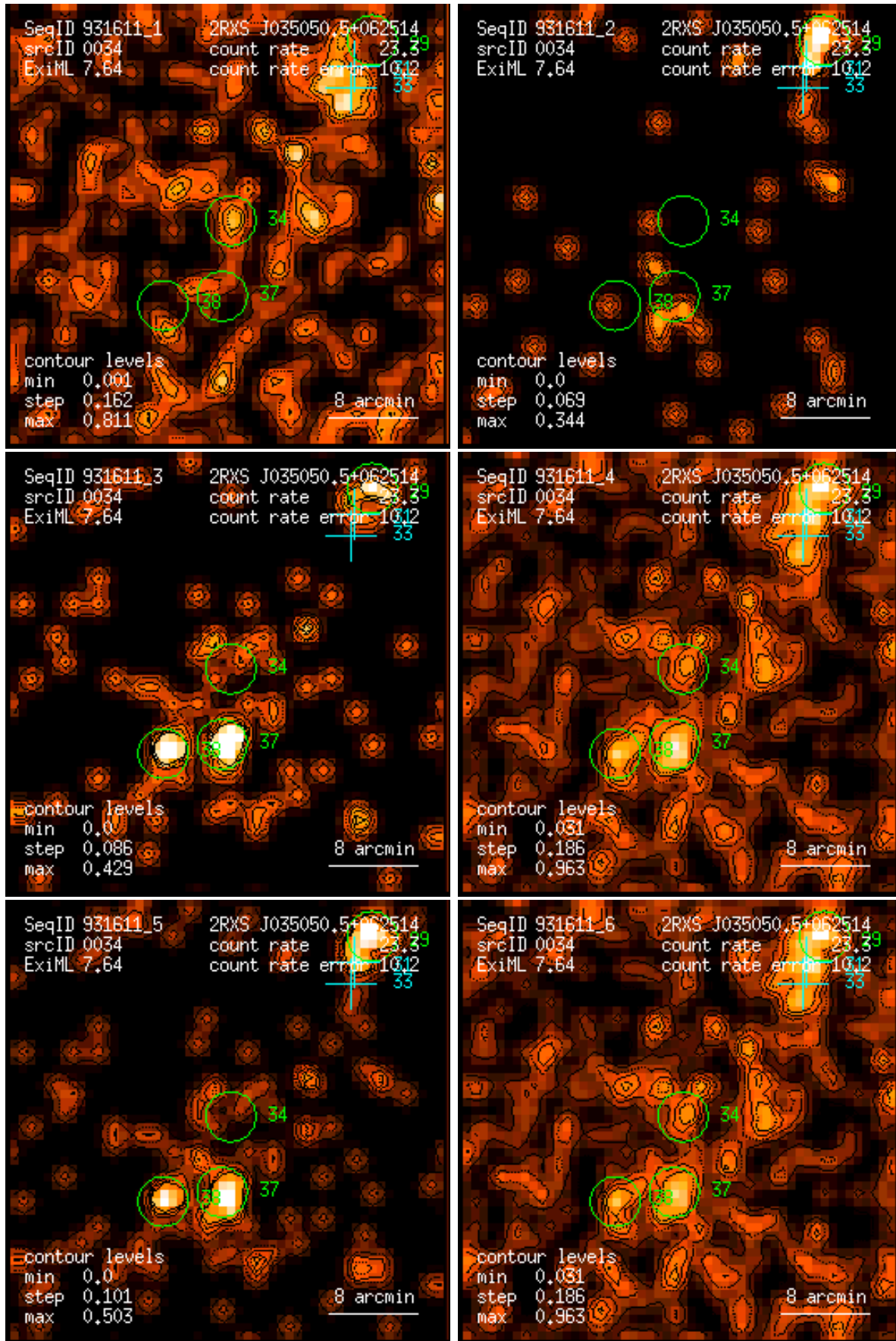
Figure 34: RASS 931611: detection 0034: band rate images, Gaussian filter: (1) PSPC channels 11 – 41, (2) 52 – 90, (3) 91 – 201, (4) 11 – 235, (5) 52 – 201, (6) 11 – 201. Broad band rates in counts/ks. Band rate contour levels in counts/ks/arcmin 2 .
