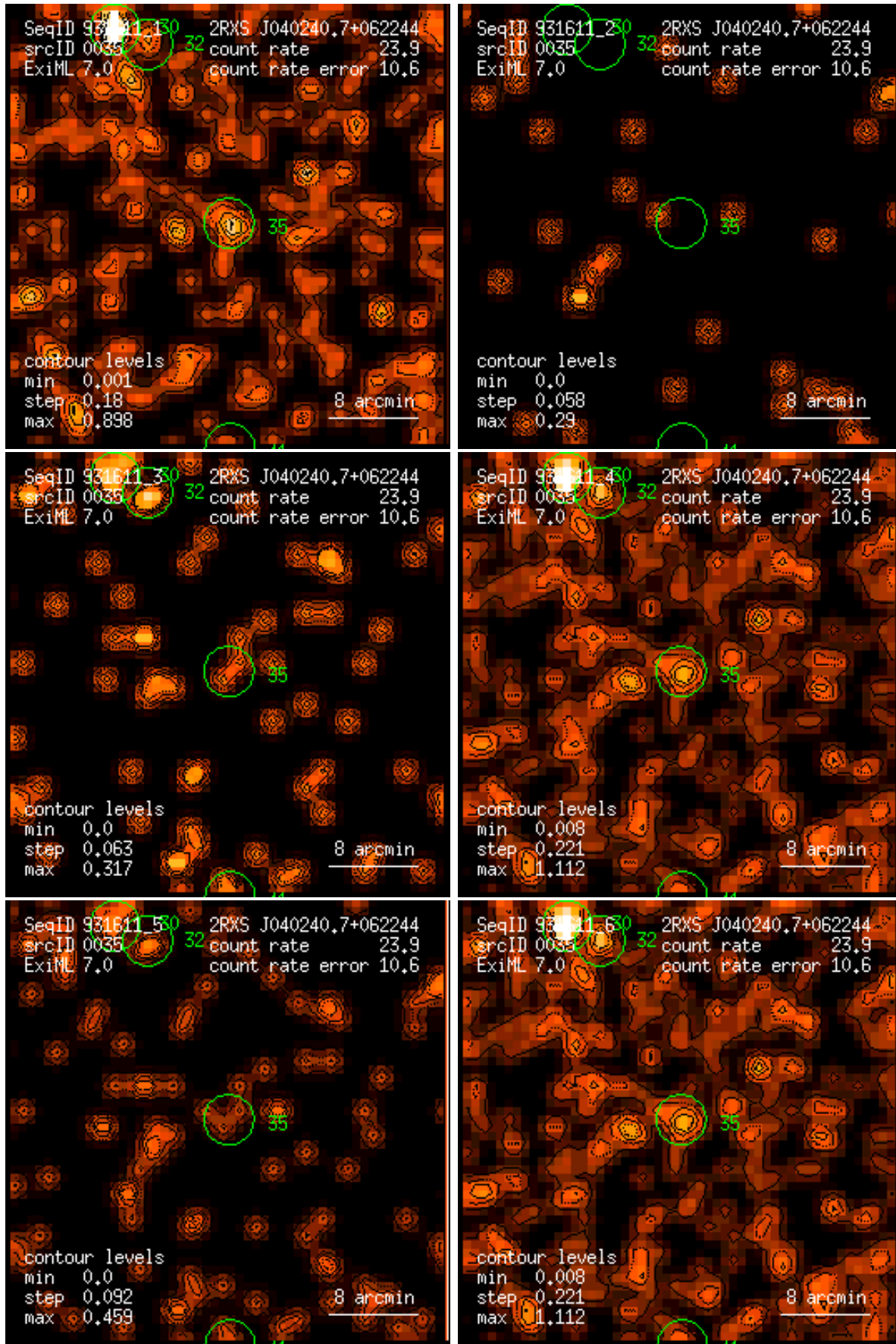
Figure 35: RASS 931611: detection 0035: band rate images, Gaussian filter: (1) PSPC channels 11 – 41, (2) 52 – 90, (3) 91 – 201, (4) 11 – 235, (5) 52 – 201, (6) 11 – 201. Broad band rates in counts/ks. Band rate contour levels in counts/ks/arcmin 2 .
