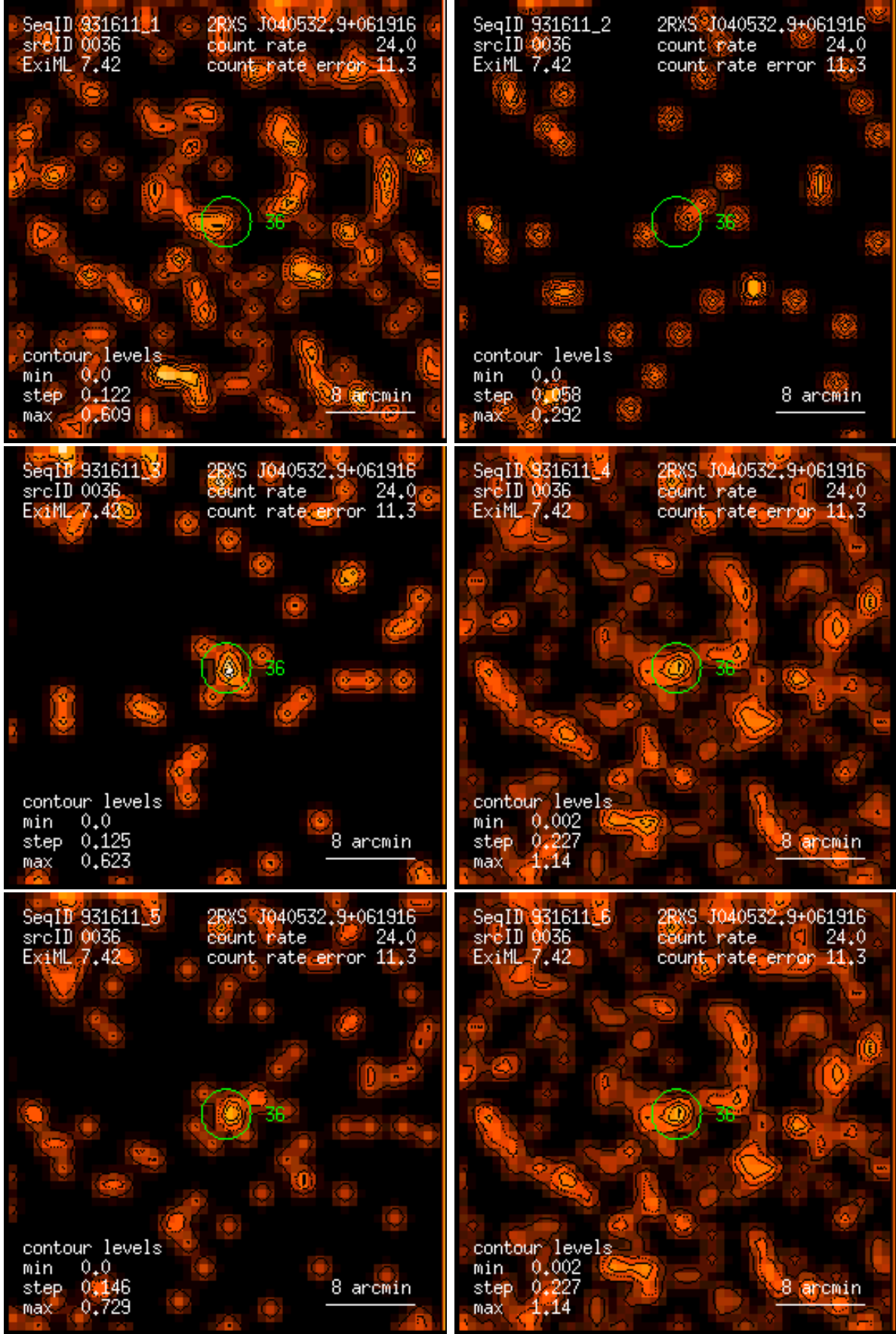
Figure 36: RASS 931611: detection 0036: band rate images, Gaussian filter: (1) PSPC channels 11 – 41, (2) 52 – 90, (3) 91 – 201, (4) 11 – 235, (5) 52 – 201, (6) 11 – 201. Broad band rates in counts/ks. Band rate contour levels in counts/ks/arcmin 2 .
