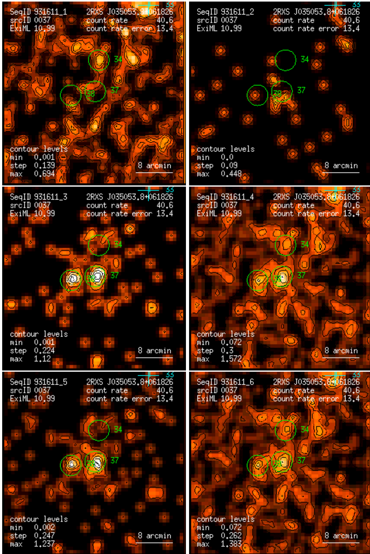
Figure 37: RASS 931611: detection 0037: band rate images, Gaussian filter: (1) PSPC channels 11 – 41, (2) 52 – 90, (3) 91 – 201, (4) 11 – 235, (5) 52 – 201, (6) 11 – 201. Broad band rates in counts/ks. Band rate contour levels in counts/ks/arcmin 2 .
