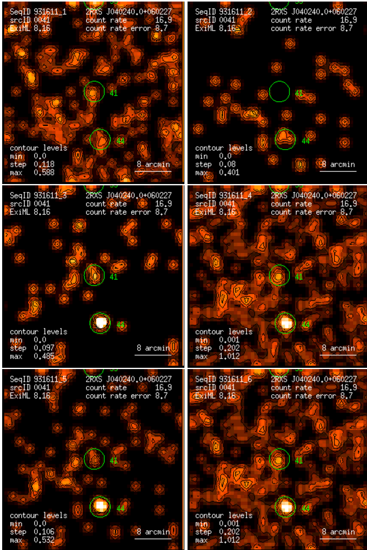
Figure 41: RASS 931611: detection 0041: band rate images, Gaussian filter: (1) PSPC channels 11 – 41, (2) 52 – 90, (3) 91 – 201, (4) 11 – 235, (5) 52 – 201, (6) 11 – 201. Broad band rates in counts/ks. Band rate contour levels in counts/ks/arcmin 2 .
