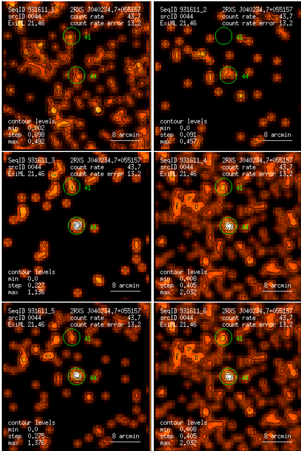
Figure 44: RASS 931611: detection 0044: band rate images, Gaussian filter: (1) PSPC channels 11 – 41, (2) 52 – 90, (3) 91 – 201, (4) 11 – 235, (5) 52 – 201, (6) 11 – 201. Broad band rates in counts/ks. Band rate contour levels in counts/ks/arcmin 2 .
