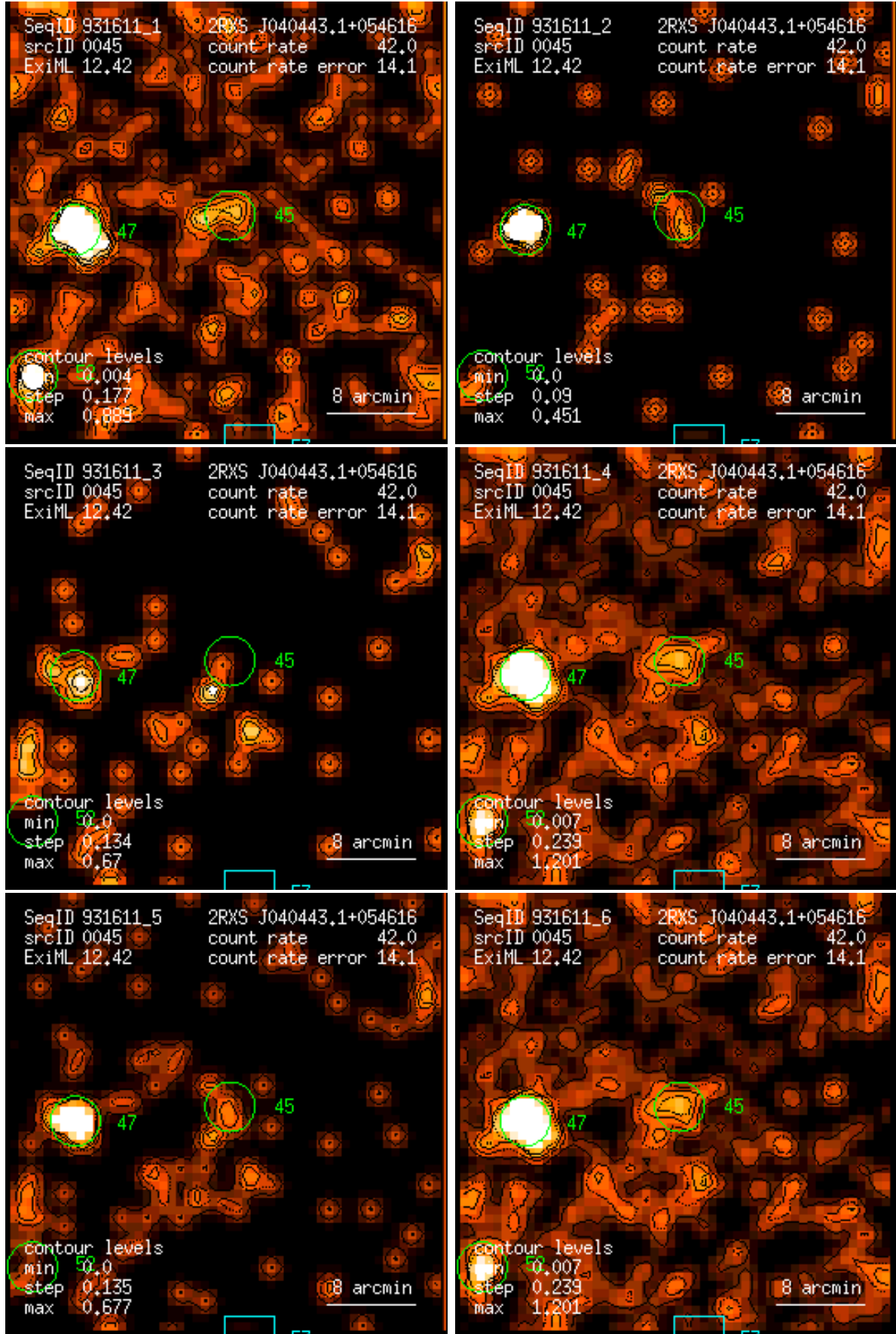
Figure 45: RASS 931611: detection 0045: band rate images, Gaussian filter: (1) PSPC channels 11 – 41, (2) 52 – 90, (3) 91 – 201, (4) 11 – 235, (5) 52 – 201, (6) 11 – 201. Broad band rates in counts/ks. Band rate contour levels in counts/ks/arcmin 2 .
