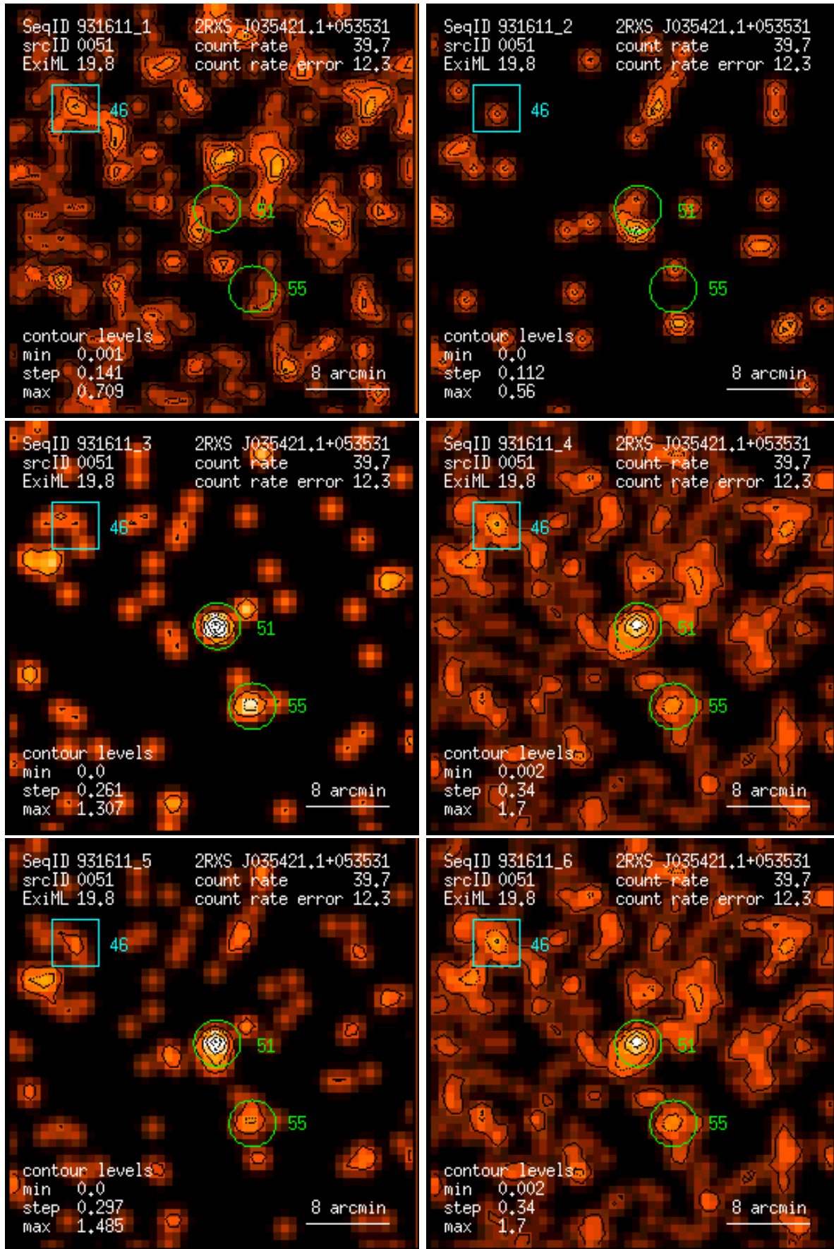
Figure 51: RASS 931611: detection 0051: band rate images, Gaussian filter: (1) PSPC channels 11 – 41, (2) 52 – 90, (3) 91 – 201, (4) 11 – 235, (5) 52 – 201, (6) 11 – 201. Broad band rates in counts/ks. Band rate contour levels in counts/ks/arcmin 2 .
