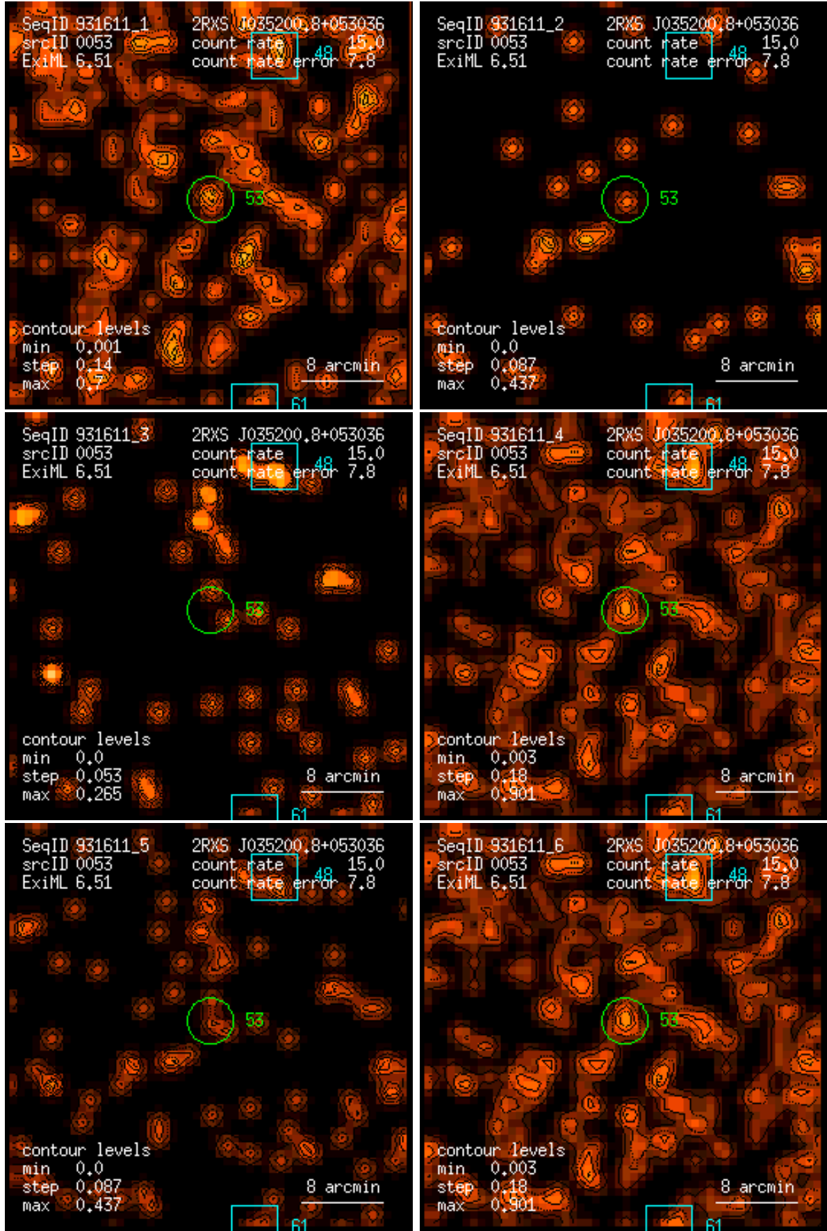
Figure 53: RASS 931611: detection 0053: band rate images, Gaussian filter: (1) PSPC channels 11 – 41, (2) 52 – 90, (3) 91 – 201, (4) 11 – 235, (5) 52 – 201, (6) 11 – 201. Broad band rates in counts/ks. Band rate contour levels in counts/ks/arcmin 2 .
