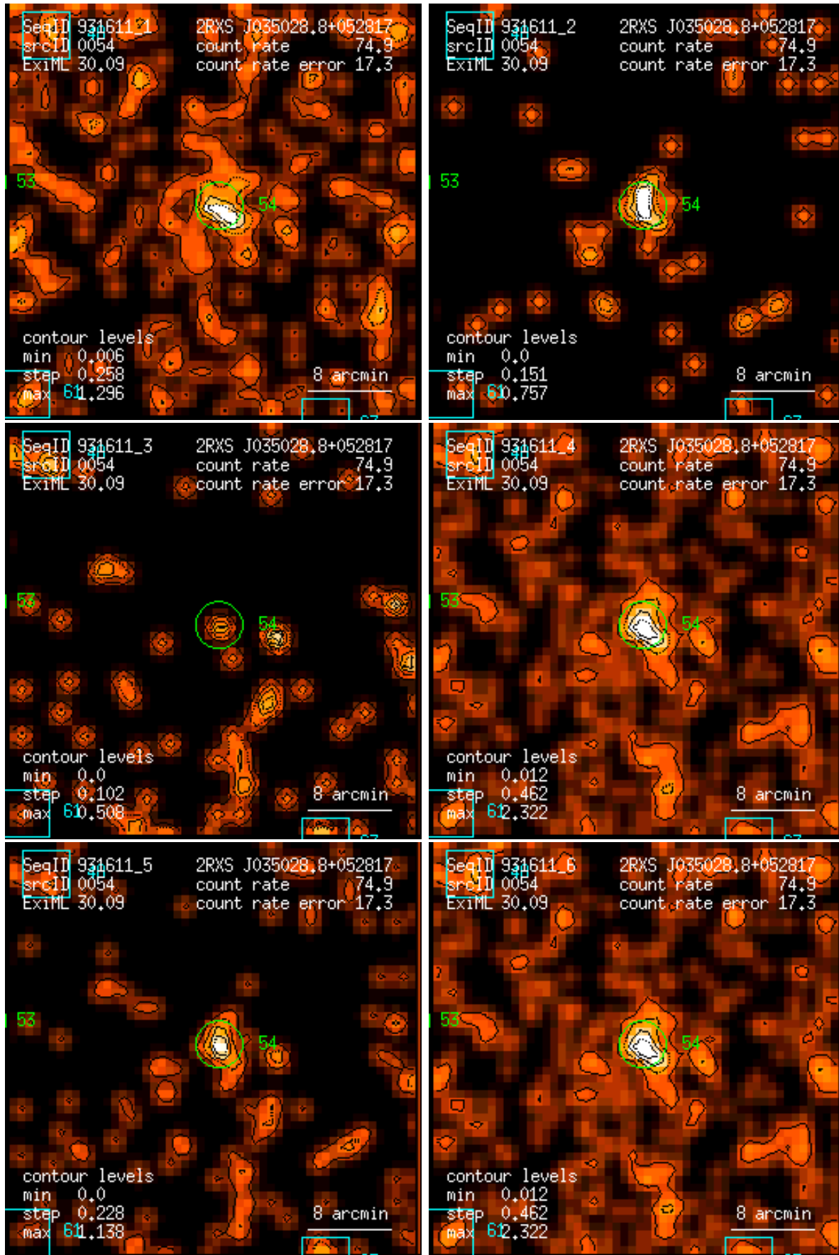
Figure 54: RASS 931611: detection 0054: band rate images, Gaussian filter: (1) PSPC channels 11 – 41, (2) 52 – 90, (3) 91 – 201, (4) 11 – 235, (5) 52 – 201, (6) 11 – 201. Broad band rates in counts/ks. Band rate contour levels in counts/ks/arcmin 2 .
