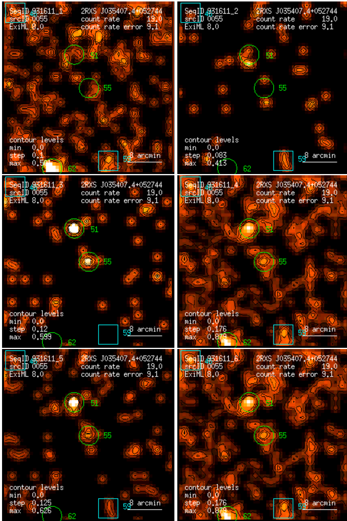
Figure 55: RASS 931611: detection 0055: band rate images, Gaussian filter: (1) PSPC channels 11 – 41, (2) 52 – 90, (3) 91 – 201, (4) 11 – 235, (5) 52 – 201, (6) 11 – 201. Broad band rates in counts/ks. Band rate contour levels in counts/ks/arcmin 2 .
