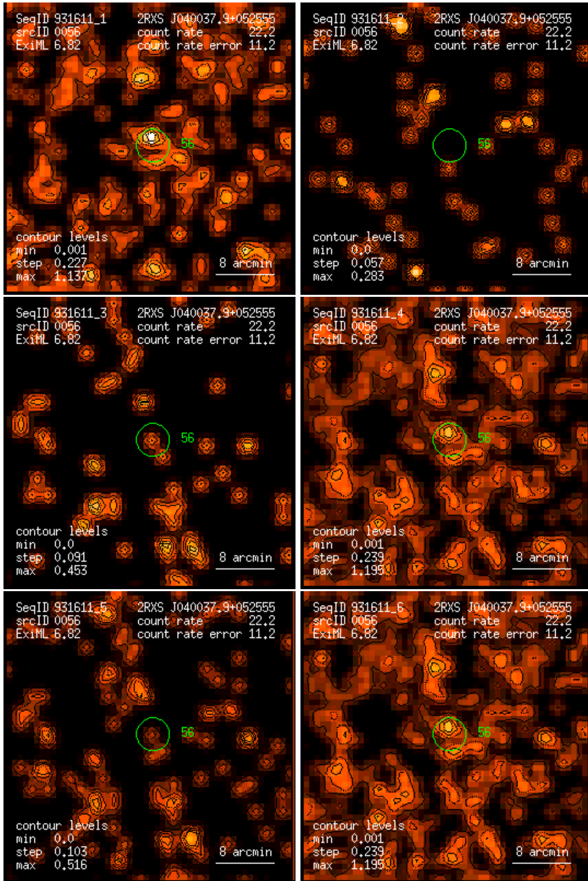
Figure 56: RASS 931611: detection 0056: band rate images, Gaussian filter: (1) PSPC channels 11 – 41, (2) 52 – 90, (3) 91 – 201, (4) 11 – 235, (5) 52 – 201, (6) 11 – 201. Broad band rates in counts/ks. Band rate contour levels in counts/ks/arcmin 2 .
