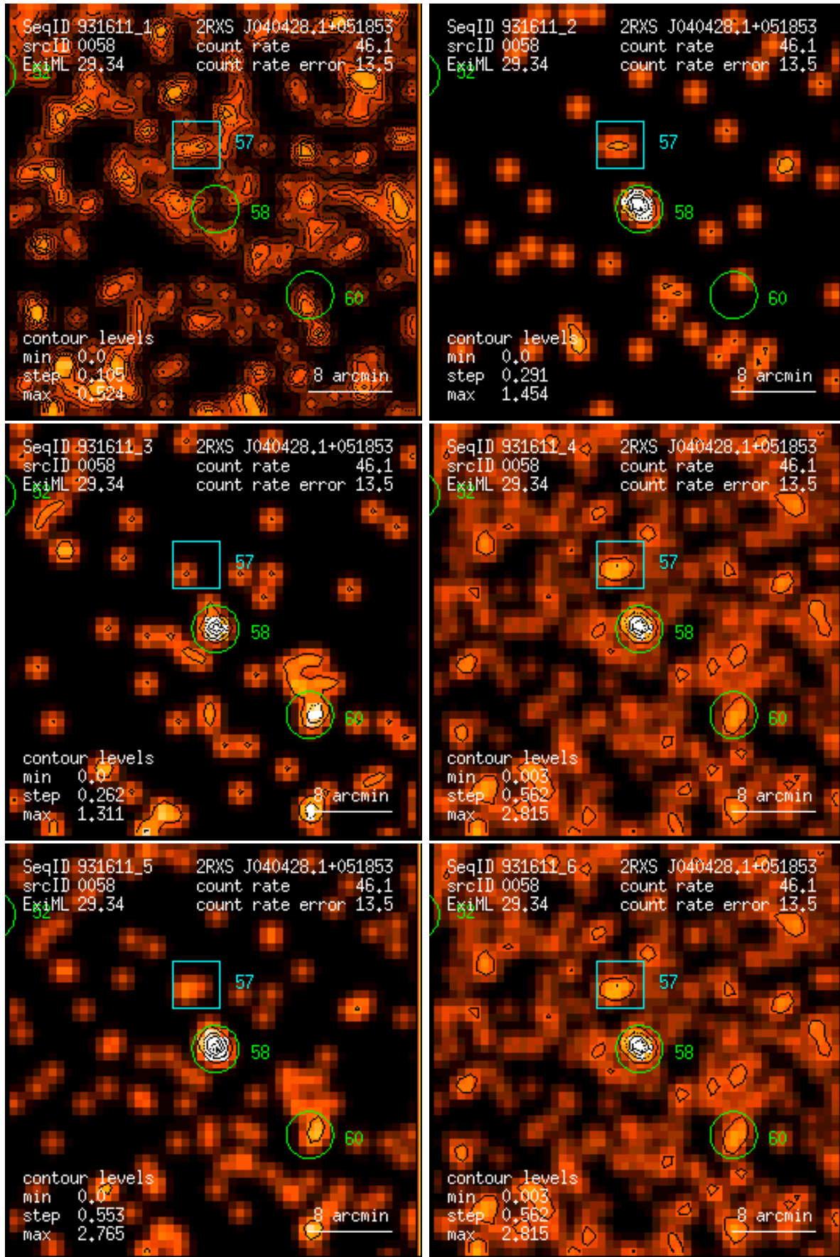
Figure 58: RASS 931611: detection 0058: band rate images, Gaussian filter: (1) PSPC channels 11 – 41, (2) 52 – 90, (3) 91 – 201, (4) 11 – 235, (5) 52 – 201, (6) 11 – 201. Broad band rates in counts/ks. Band rate contour levels in counts/ks/arcmin 2 .
